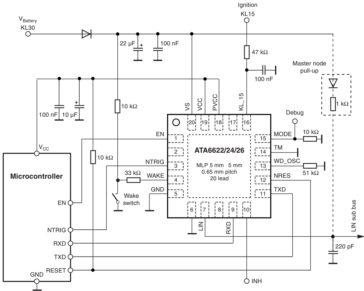
Figure 9-2. Application Circuit
