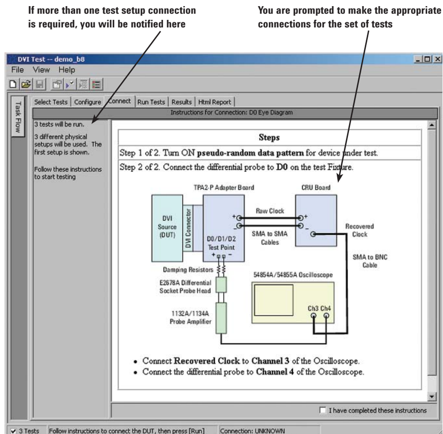
Figure 4. When you make multiple tests where the connections must be changed, the software prompts you with connection diagrams and/or photographs.
