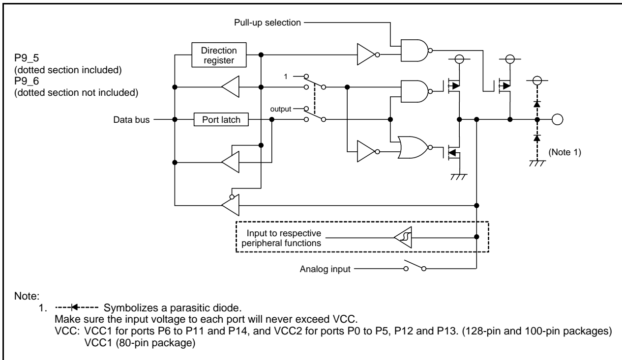
Figure 13.8 I/O Ports (8/9)
