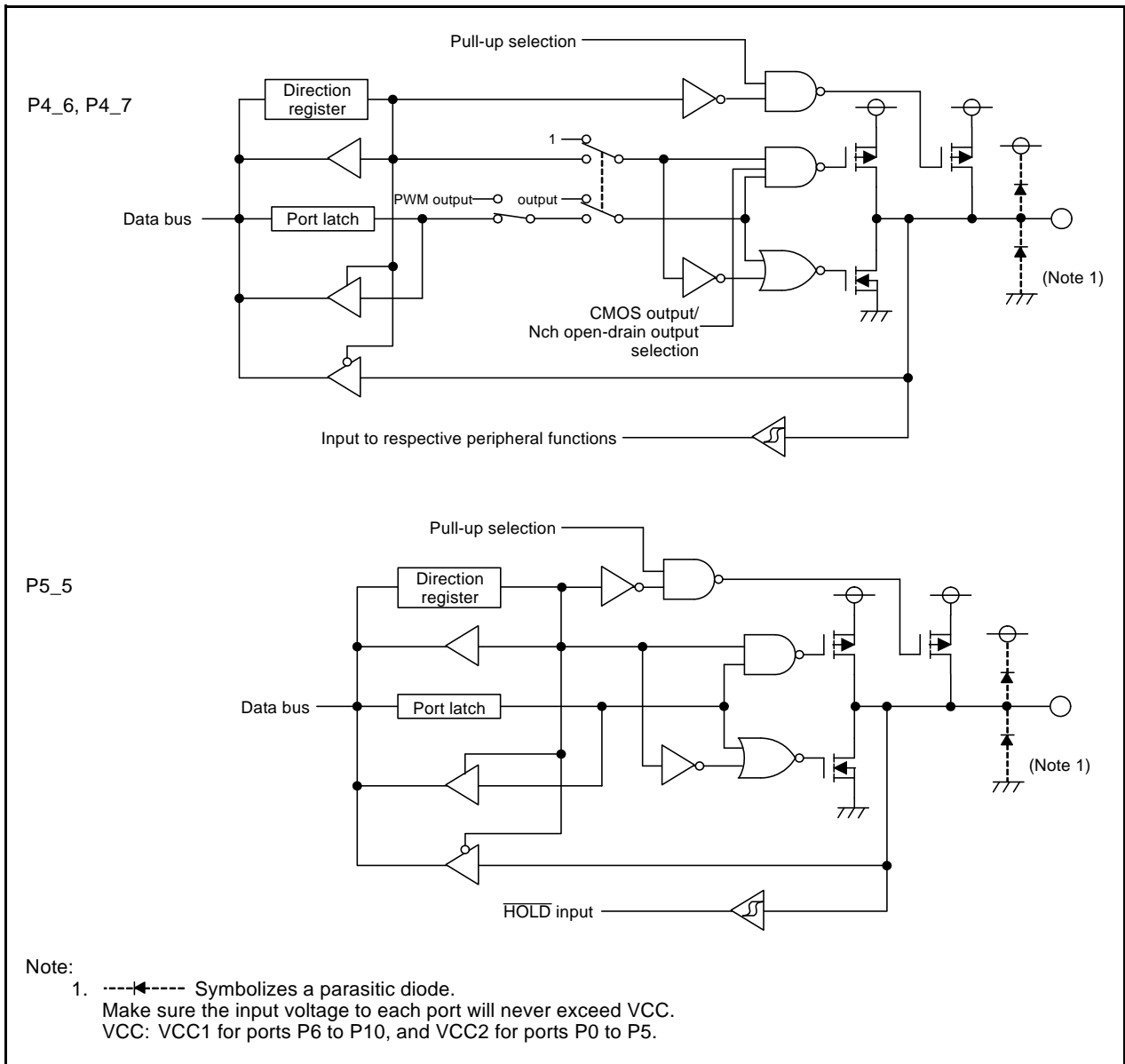
Figure 13.5 I/O Ports (5/9)
