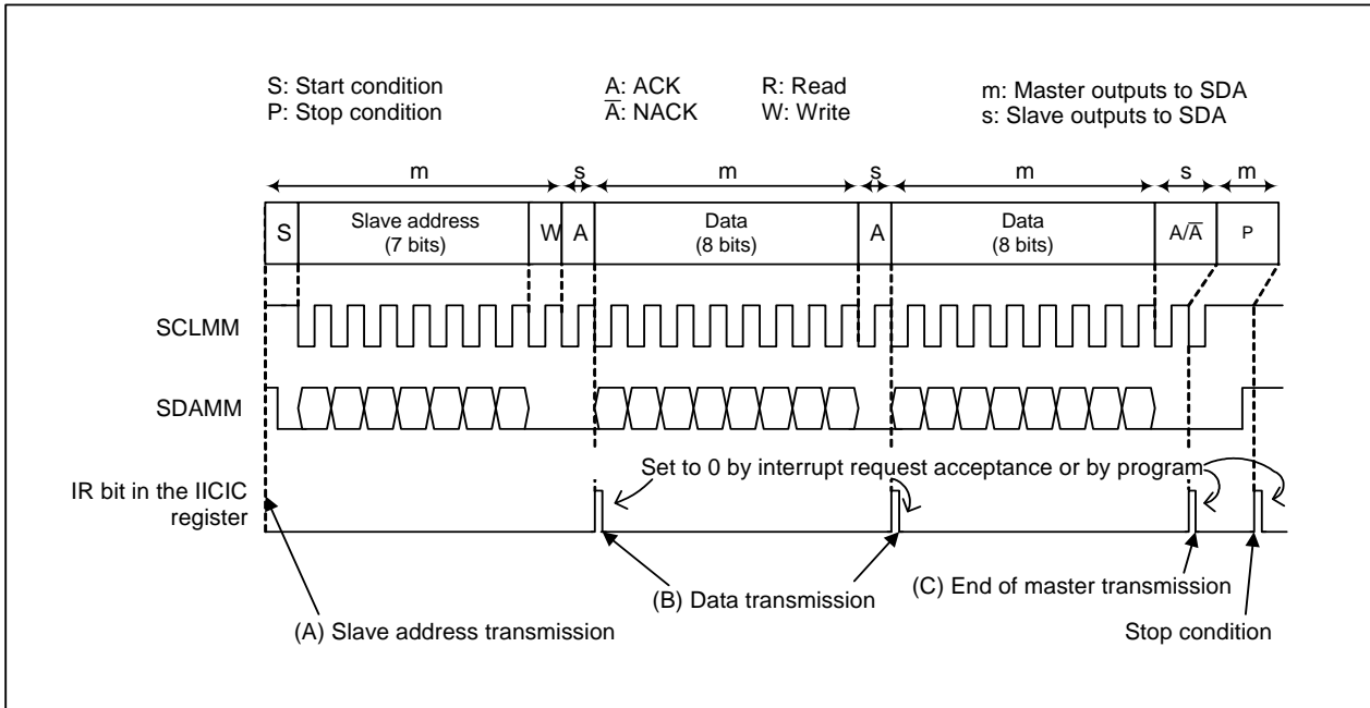
Figure 25.17 Example of Master Transmission
