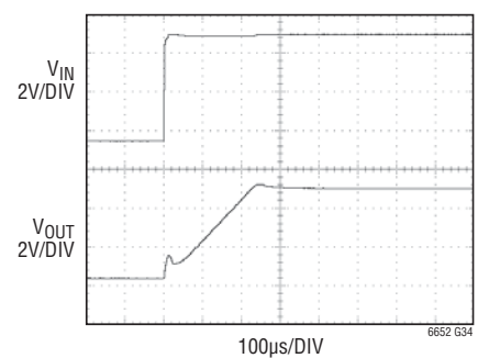
5V Start-Up Response with Output Capacitor
