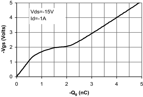
Figure 7: Gate-Charge Characteristics
