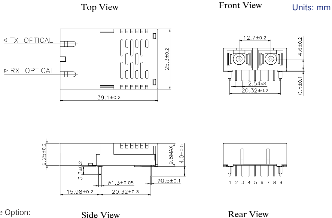
Package Diagram (9.8 mm SC transceiver assembly)
