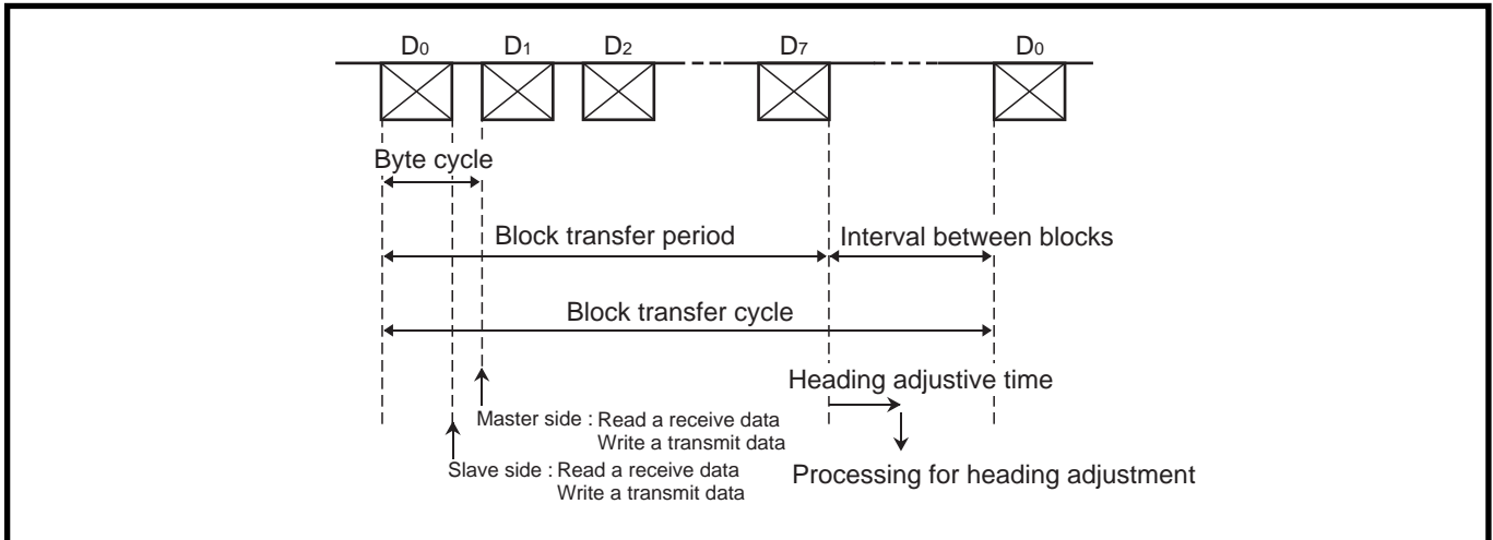
Fig. 2.3.33 Timing chart [Cyclic transmission or reception of block data between microcomputers]
