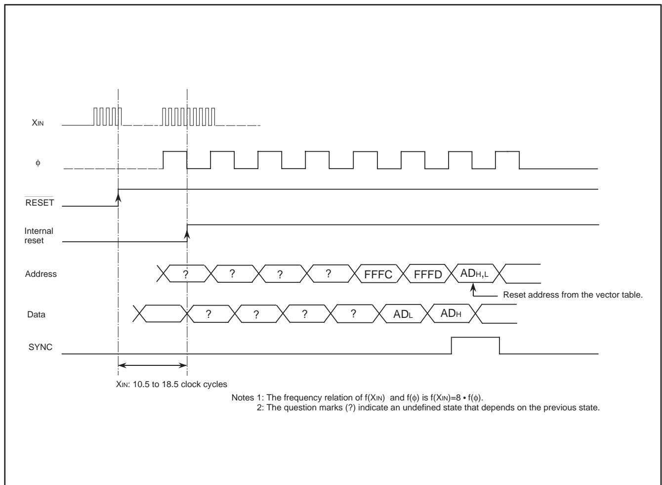
Fig. 55. Reset sequence
