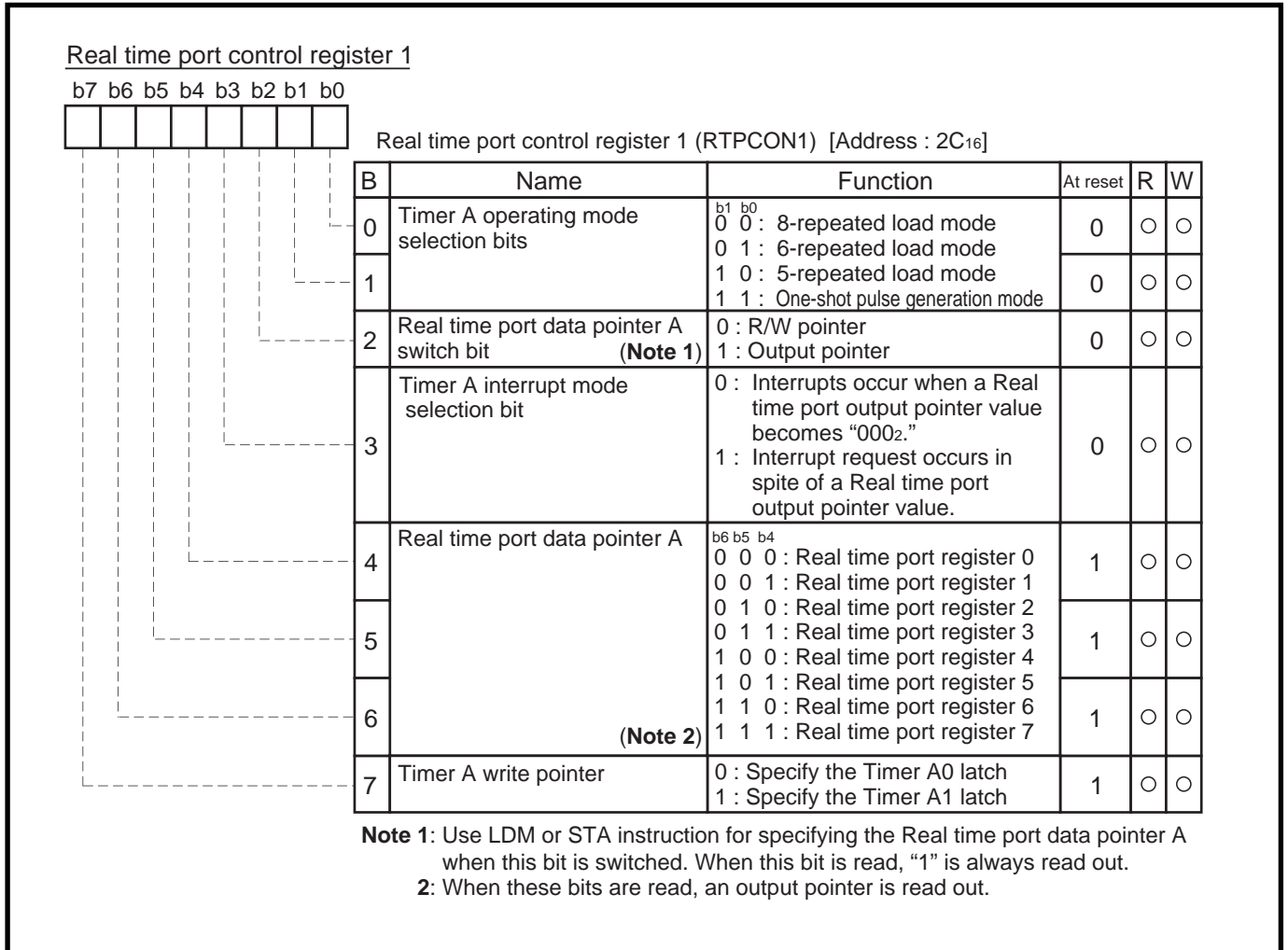
Fig. 2.4.4 Structure of Real time port control register 1
