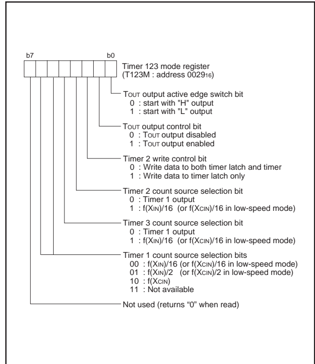
Fig. 26. Structure of Timer 123 mode register
