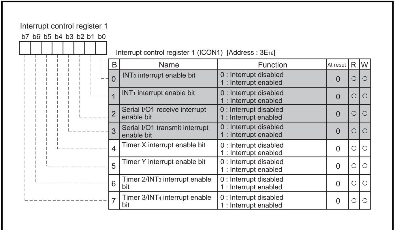
Fig. 2.2.12 Structure of Interrupt control register 1
