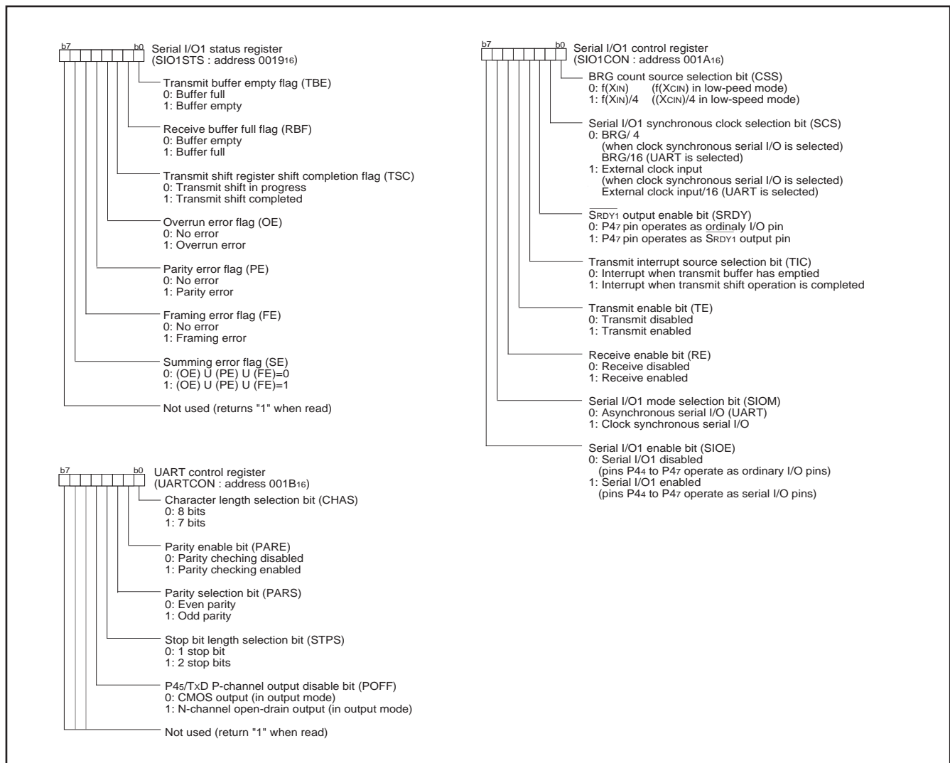
Fig. 39. Structure of serial I/O1 related register
