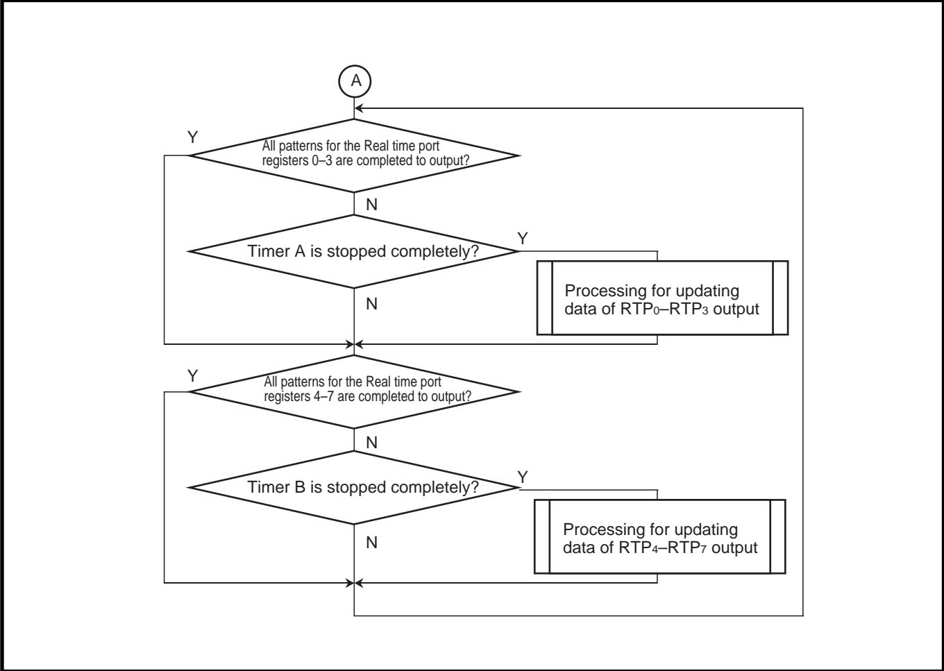
Fig. 2.4.20 Control procedure (2)
