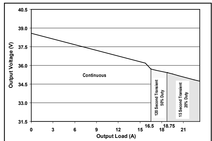
Figure 6: 36 V OUT droop characteristics.
