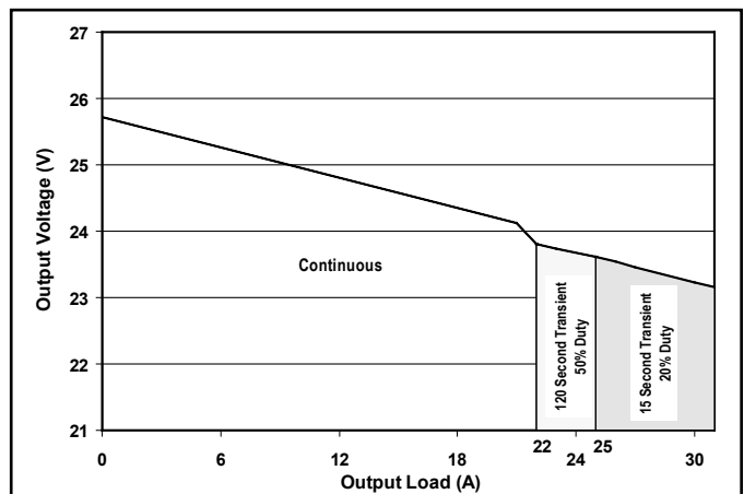
Figure 4: 24 V OUT droop characteristics.
