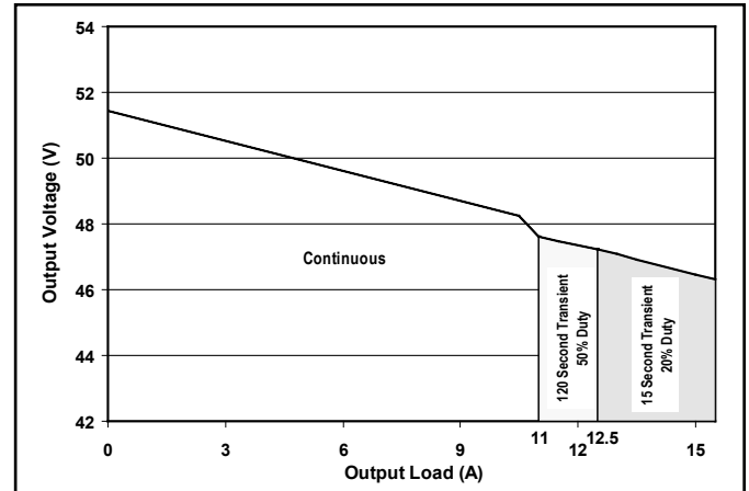
Figure 8: 48 V OUT droop characteristics.
