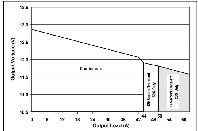
Figure 2: 12 V OUT droop characteristics.
