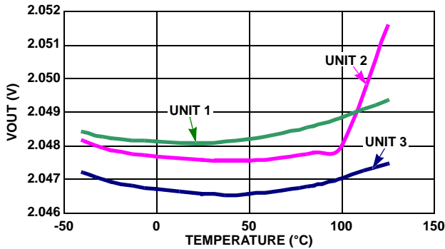
FIGURE 47. V_{OUT} VS TEMPERATURE, 3 UNITS
