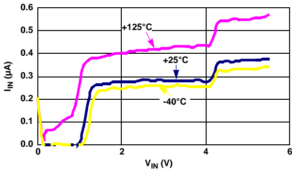
FIGURE 19. I_{IN} vs V_{IN} [SLEEP MODE], 3 TEMPERATURES
