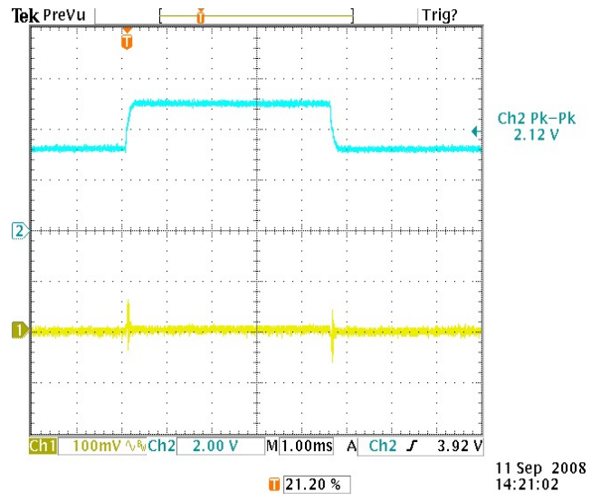
FIGURE 28. LOAD TRANSIENT RESPONSE, 100nF LOAD CAPACITANCE
