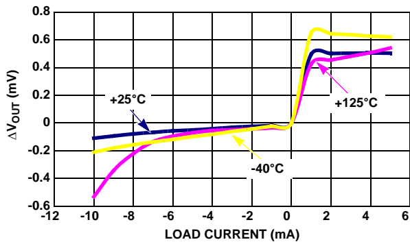
FIGURE 21. LOAD REGULATION
