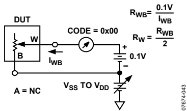
Figure 39. Wiper Resistance
