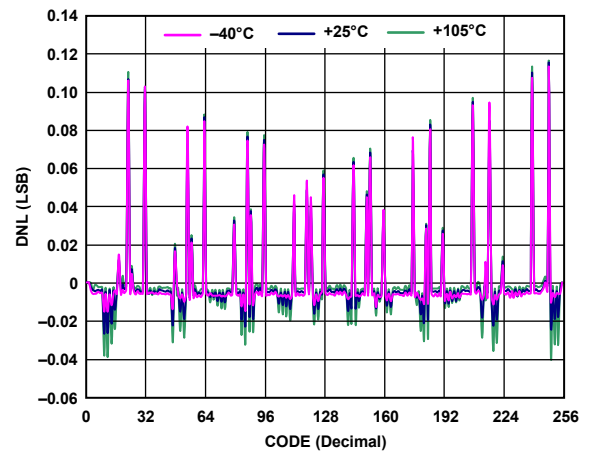
Figure 17. DNL in R-Perf Mode vs. Code vs. Temperature (AD5291)
