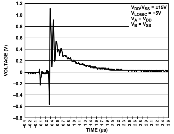
Figure 33. Maximum Transition Glitch
