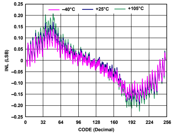
Figure 16. INL in R-Perf Mode vs. Code vs. Temperature (AD5291)
