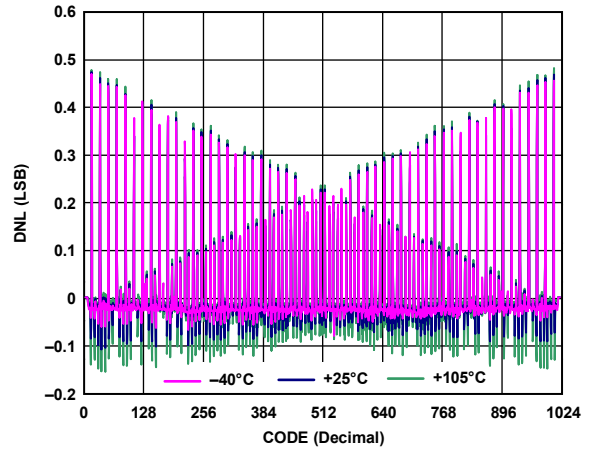
Figure 15. DNL in R-Perf Mode vs. Code vs. Temperature (AD5292)
