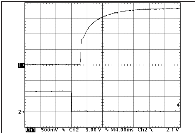
Figure 9: Turn-on transient at full load (resistive load) (4 ms/div). Ch 1: V out (500mV/div) Ch 2: ON/OFF input (5V/div)
