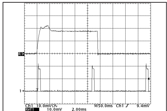
Figure 18: Load current (10A/div) as a function of time when the converter attempts to turn on into a 10\ \text{m}\Omega short circuit. Top trace ( 2.0\ \text{ms}/\text{div} ) is an expansion of the on-time portion of the bottom trace.
