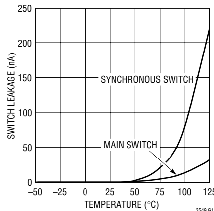
Switch Leakage vs Temperature VIN = 5.5V
