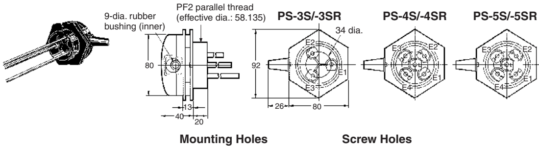
Mounting Holes
