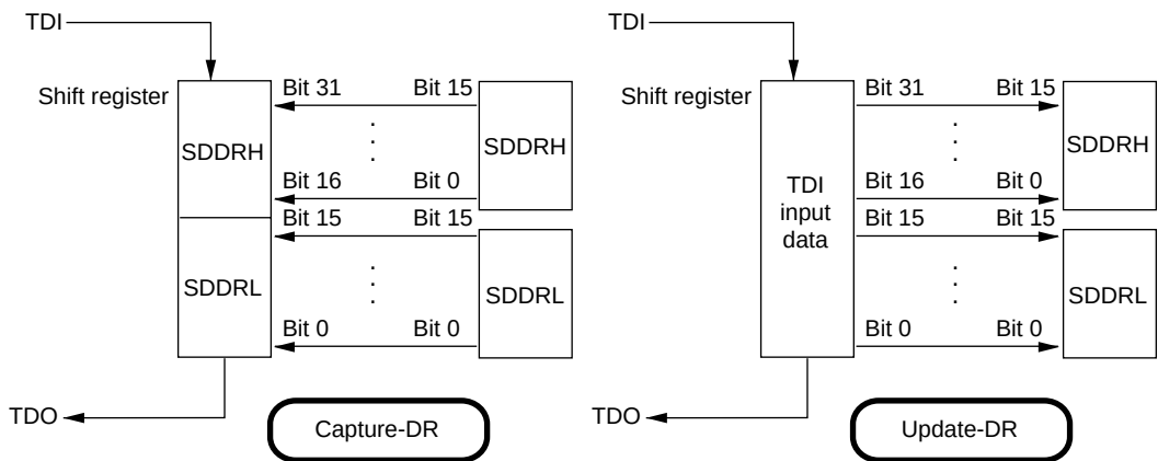
Figure 18.6 Serial Data Input/Output (2)
