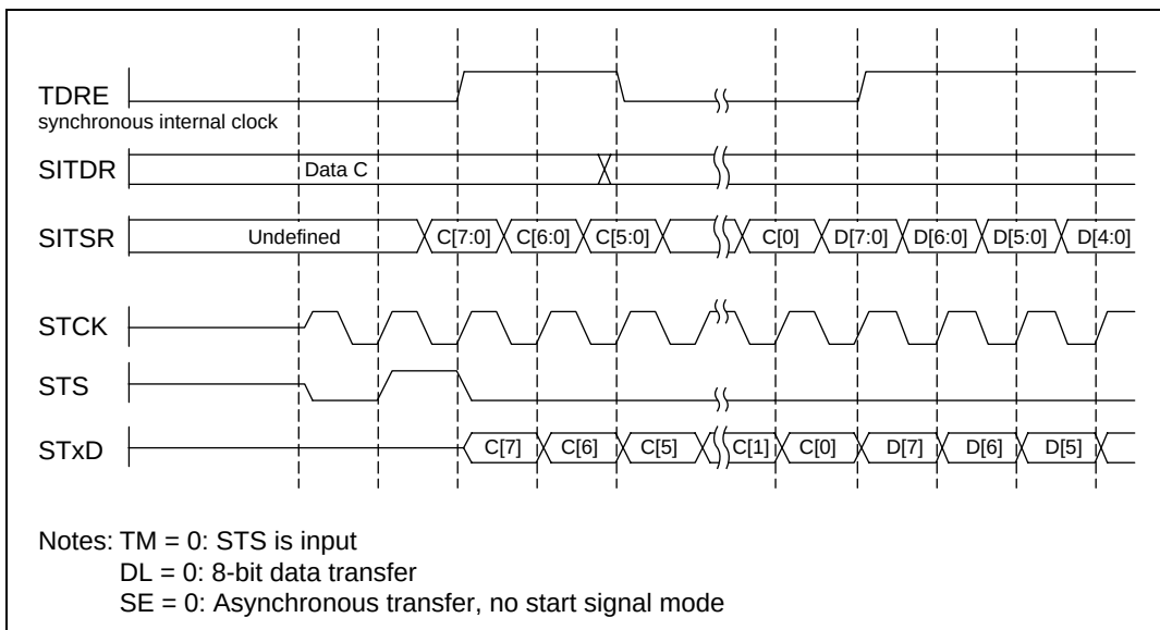
Figure 16.5 Transmission: Continuous Transfer Mode (TM = 0 Mode)
