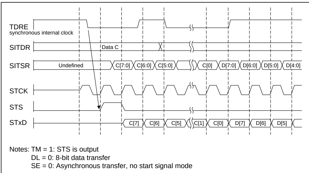
Figure 16.7 Transmission: Continuous Transfer Mode (TM = 1 Mode)
