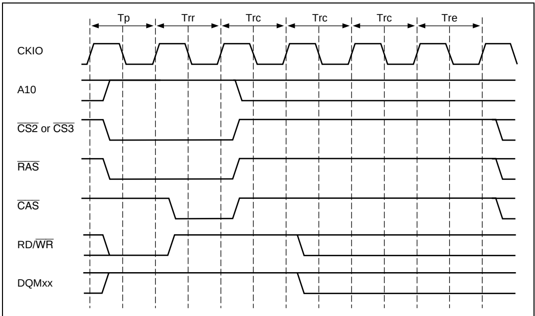
Figure 7.33 Auto-Refresh Timing
