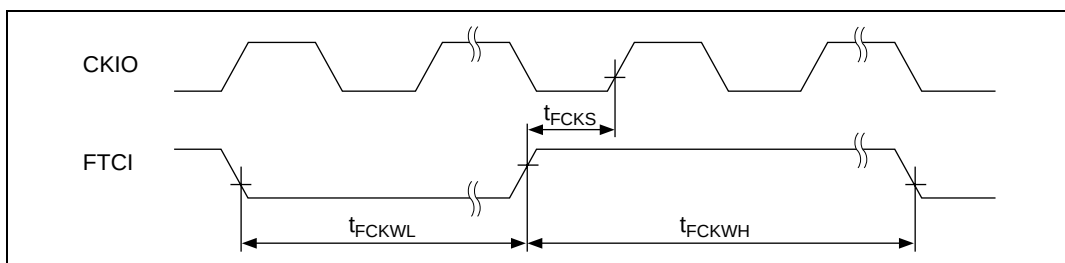
Figure 22.50 FRT Clock Input Timing ( t_{Eyc}:t_{Pyc} = 1:1 )
