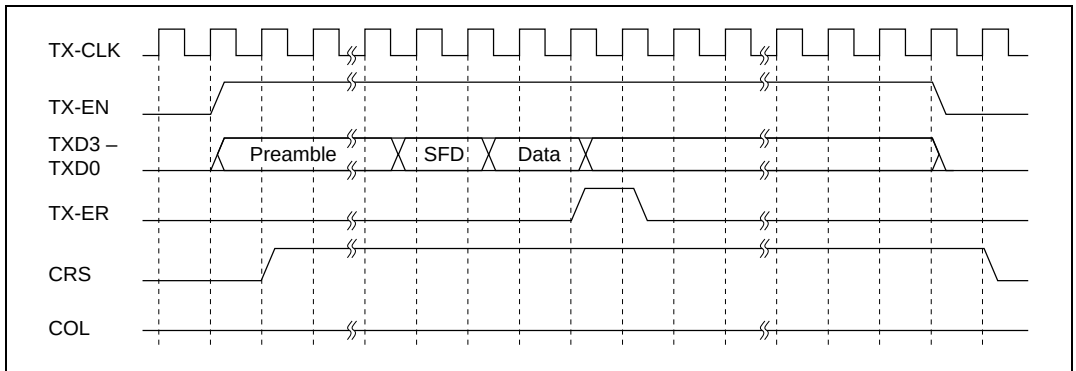
Figure 9.4 (c) MII Frame Transmit Timing (Transmit Error)
