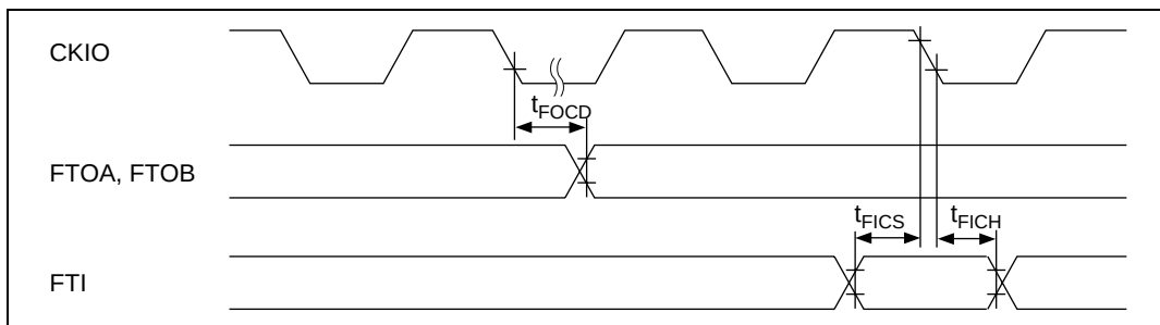
Figure 22.49 FRT Input/Output Timing ( t_{Eyc}:t_{Pyc} other than 1:1)
