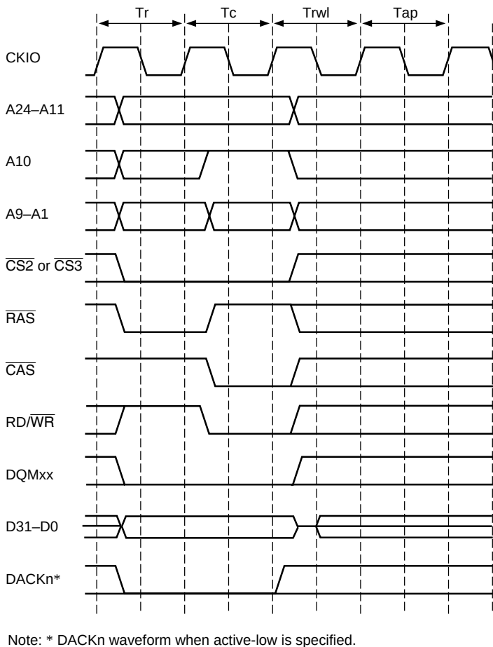
Figure 7.25 Basic Single Write Cycle Timing (Auto-Precharge)
