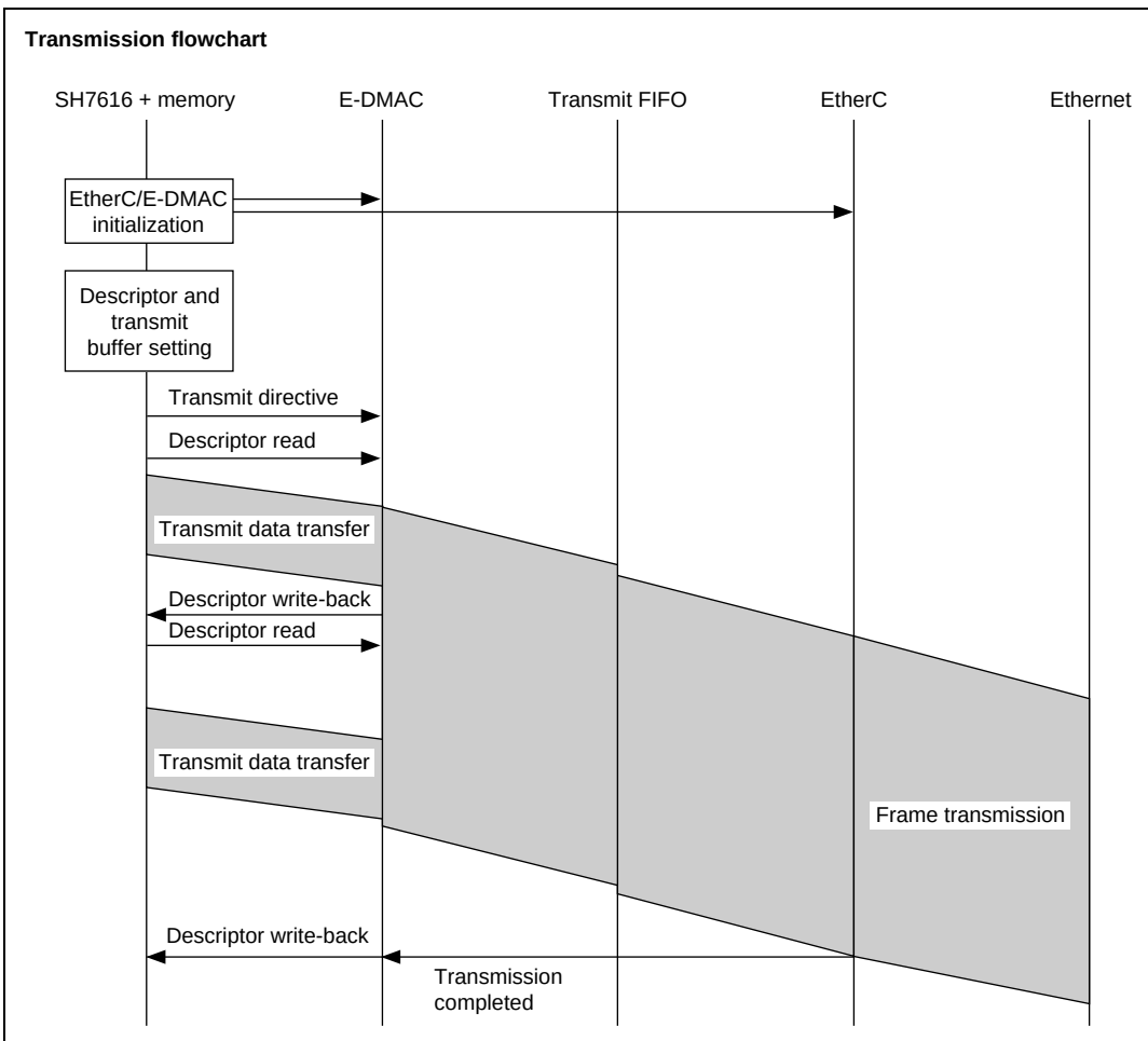
Figure 10.4 Sample Transmission Flowchart
