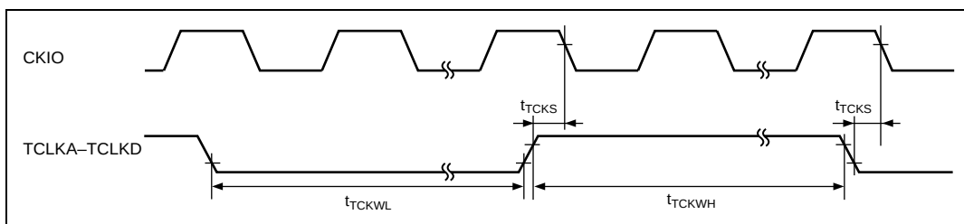
Figure 22.57 TPU Clock Input Timing
