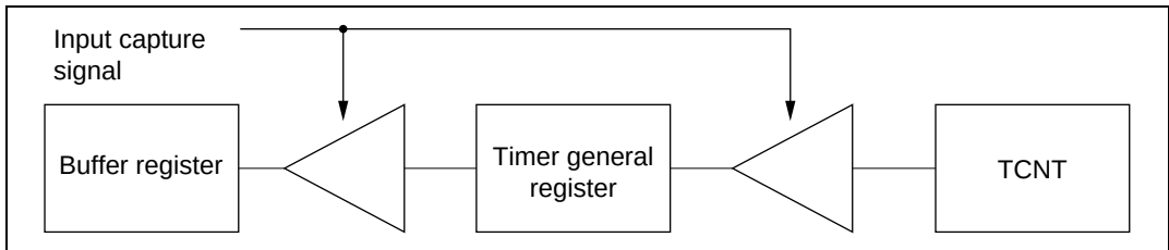
Figure 17.17 Input Capture Buffer Operation
