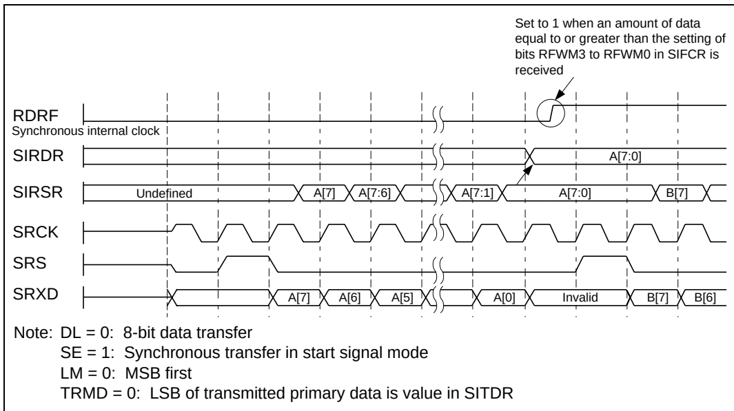
Figure 15.2 Reception: Interval Transfer Mode/MSB First
