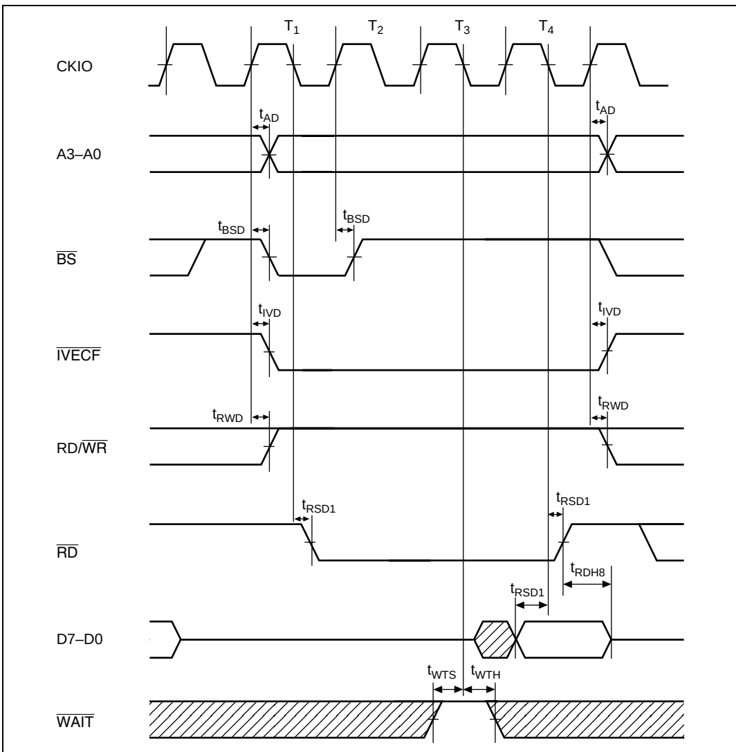
Figure 22.43 Interrupt Vector Fetch Cycle (No Wait, I\phi:E\phi = 1:1 )
