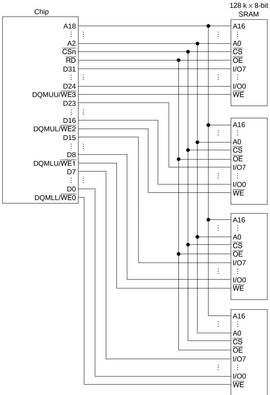
Figure 7.13 Example of 32-Bit Data Width SRAM Connection
