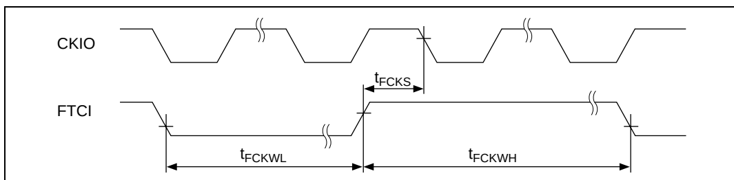
Figure 22.51 FRT Clock Input Timing ( t_{Eyc}:t_{Pyc} other than 1:1)
