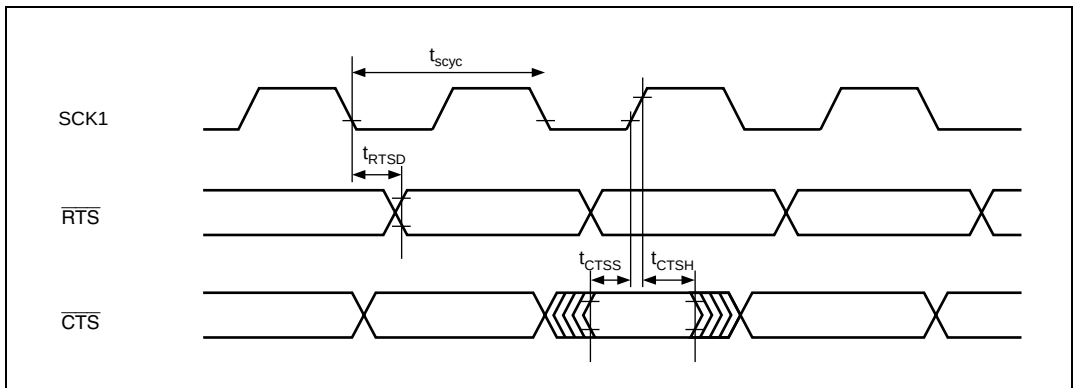
Figure 22.54 \overline{\text{RTS}} and \overline{\text{CTS}} Input/Output Timing
