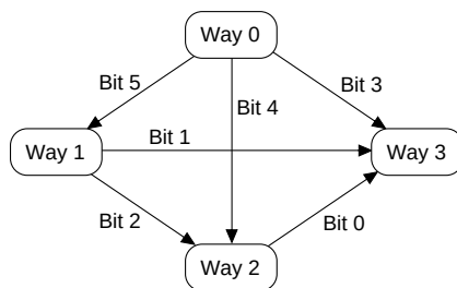
Figure 8.10 LRU Information and Access Sequence
