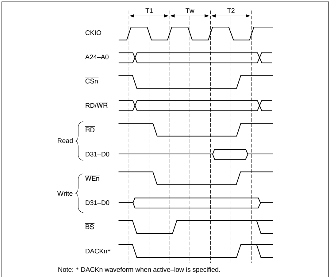
Figure 7.16 Wait Timing of Ordinary Space Access (Software Wait Only)
