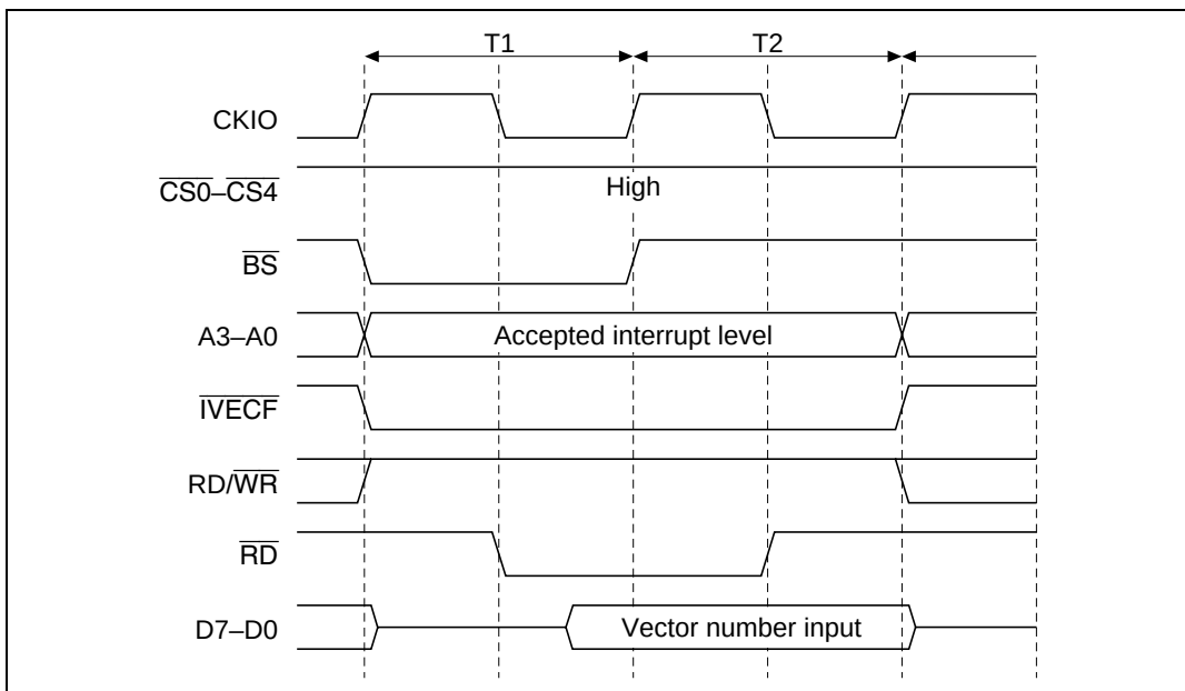
Figure 5.5 External Vector Fetch ( I\phi : E\phi \neq 1 : 1 )
