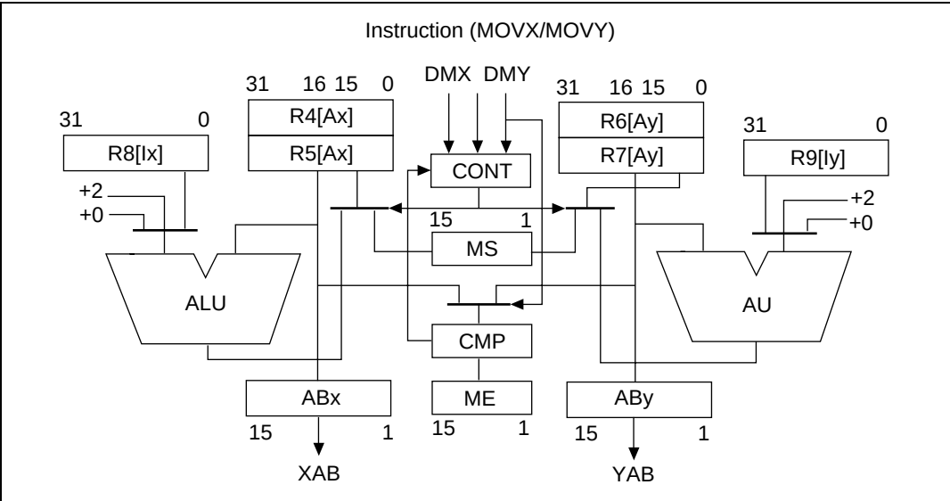
Figure 2.11 Modulo Addressing
