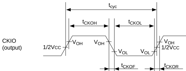
Figure 22.3 CKIO Clock Output Timing
