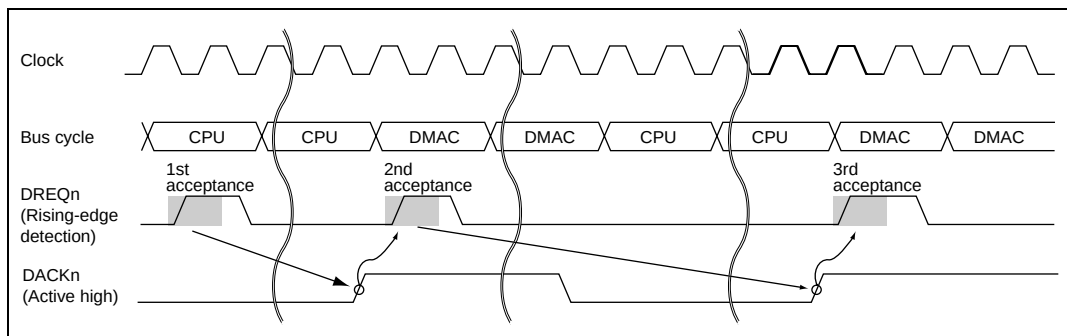
Figure 11.33 DREQn/DACKn Handshaking
