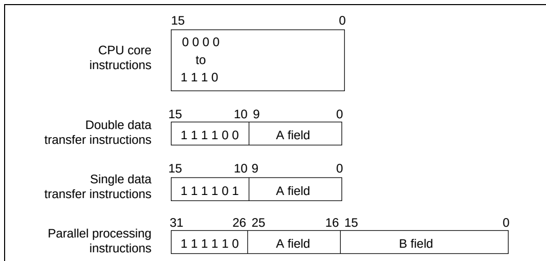
Figure 2.12 Instruction Formats for DSP Instructions
