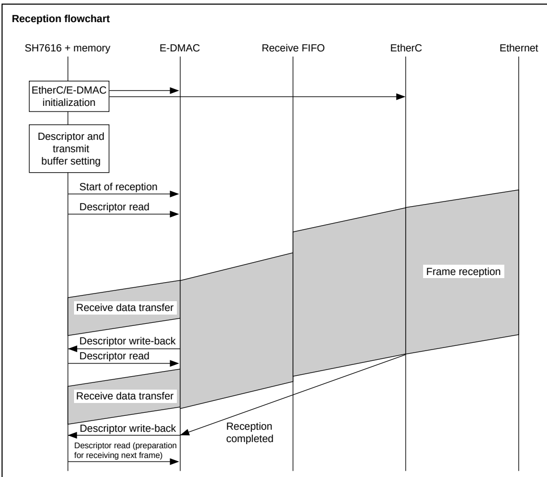
Figure 10.5 Sample Reception Flowchart
