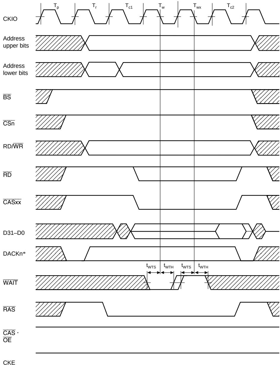
Figure 22.36 DRAM Bus Cycle (TRP = 1 Cycle, RCD = 1 Cycle, External Wait Input)
