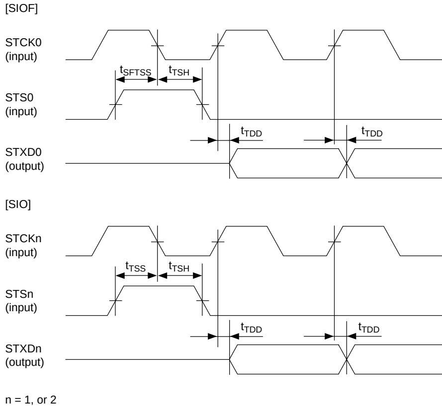
Figure 22.62 SIOF / SIO Transmit Timing (TMn = 0 Mode)
