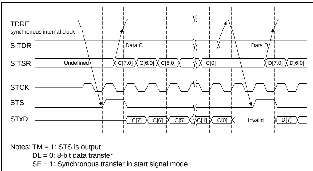
Figure 16.6 Transmission: Interval Transfer Mode (TM = 1 Mode)
