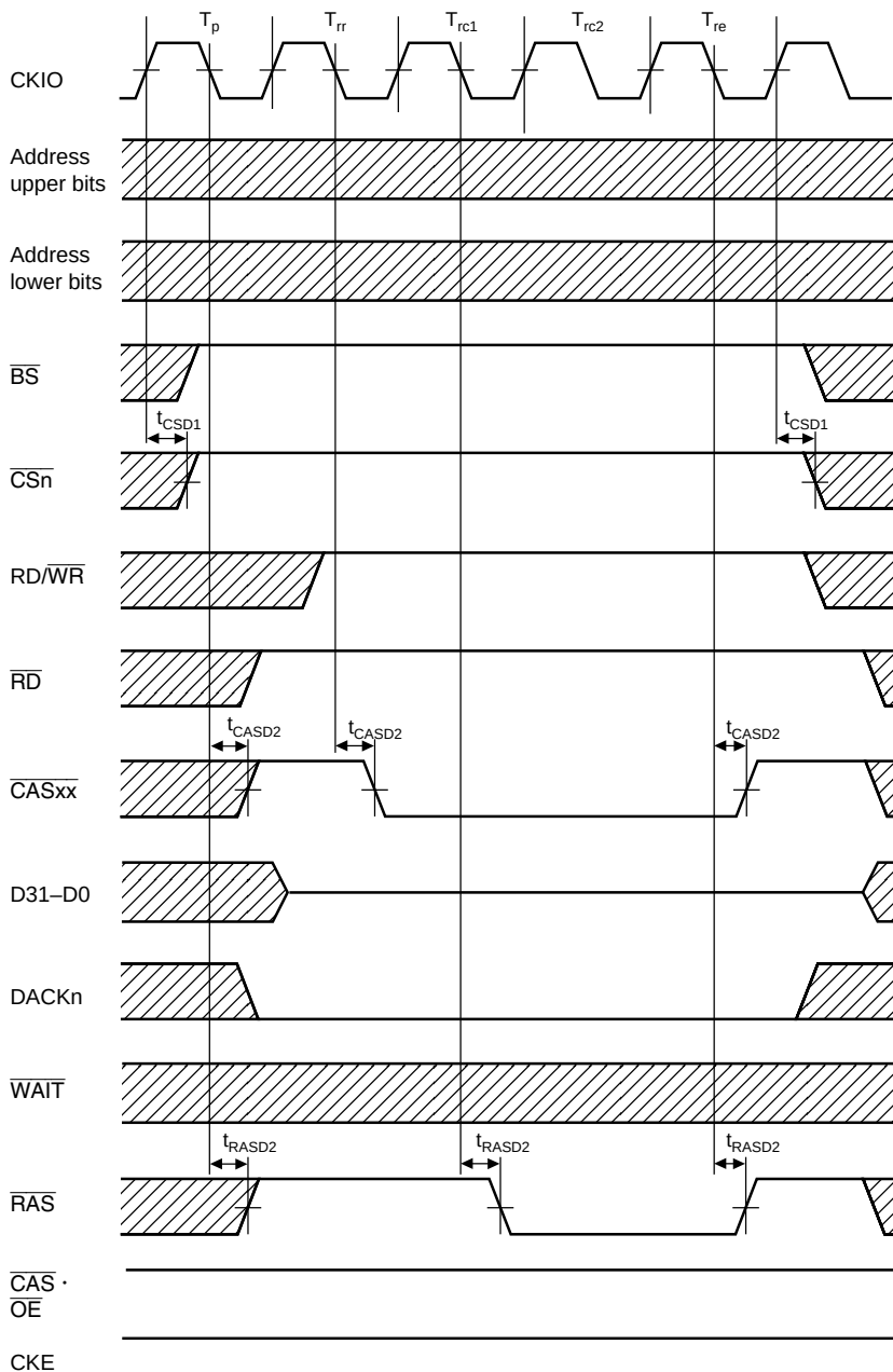
Figure 22.41 DRAM \overline{\text{CAS}} -Before- \overline{\text{RAS}} Refresh Cycle (TRP = 1 Cycle, TRAS = 2 Cycles)
