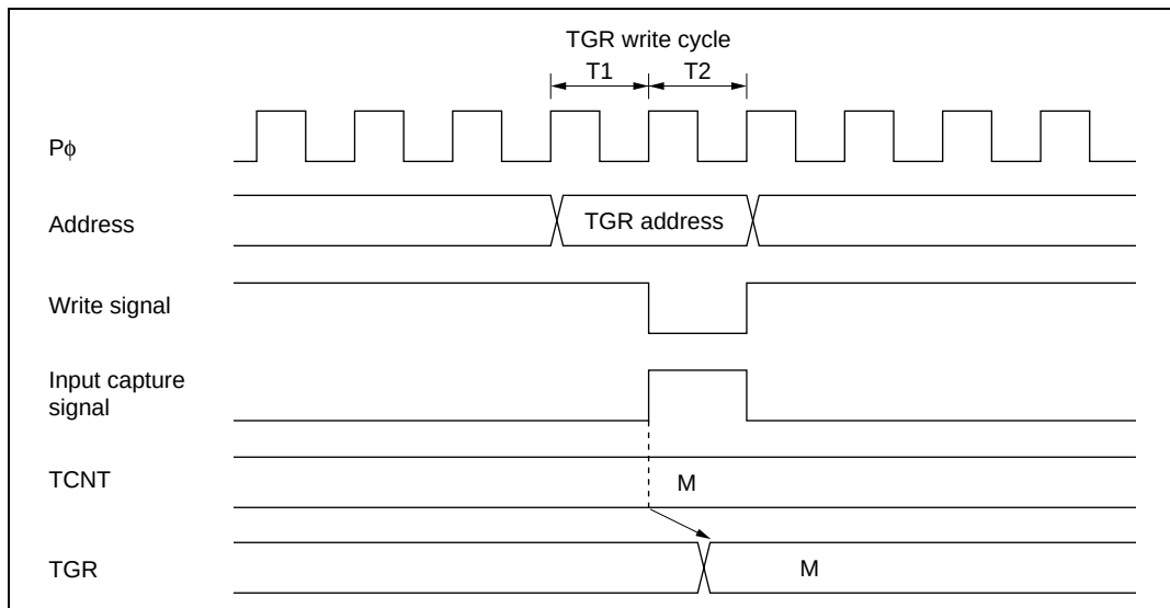
Figure 17.50 Contention between TGR Write and Input Capture
