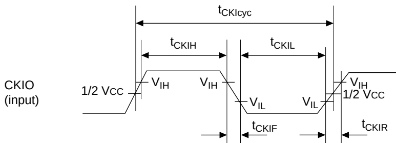
Figure 22.2 CKIO Clock Input Timing
