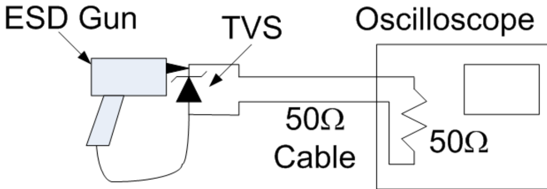
Figure 4. Diagram of ESD Test Setup
