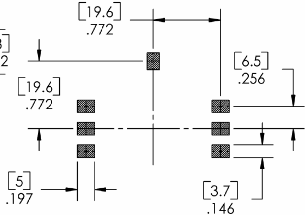
PRINTED CIRCUIT BOARD FOOTPRINT
