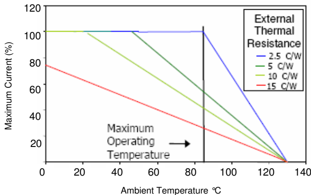
Derating Curves - Blue, Green and White LEDs
