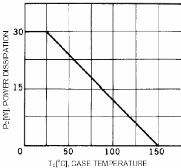
Fig.7 Power Derating
