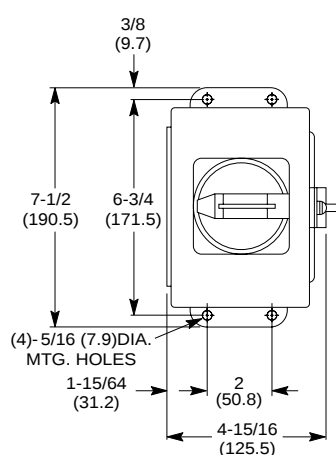
Dim Ref. A1 194E-CA20...63, 194E-FA20...63, 194E-AA20...63
