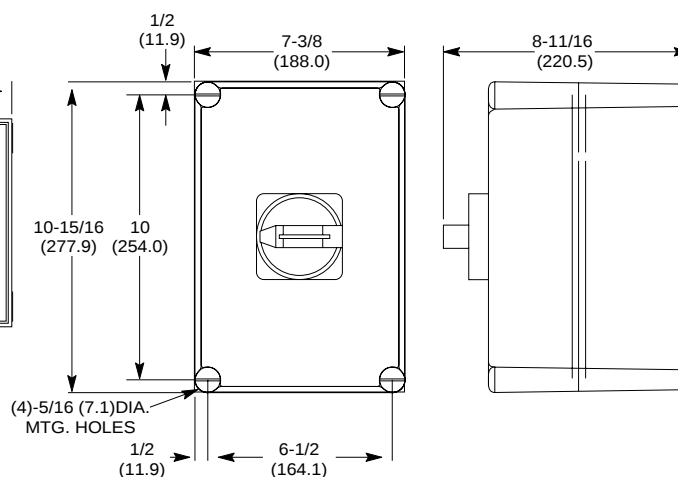
Dim Ref. B1 194E-KA80...00
