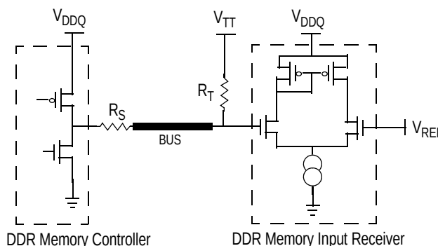
Figure 6. DDR System Level Diagram
