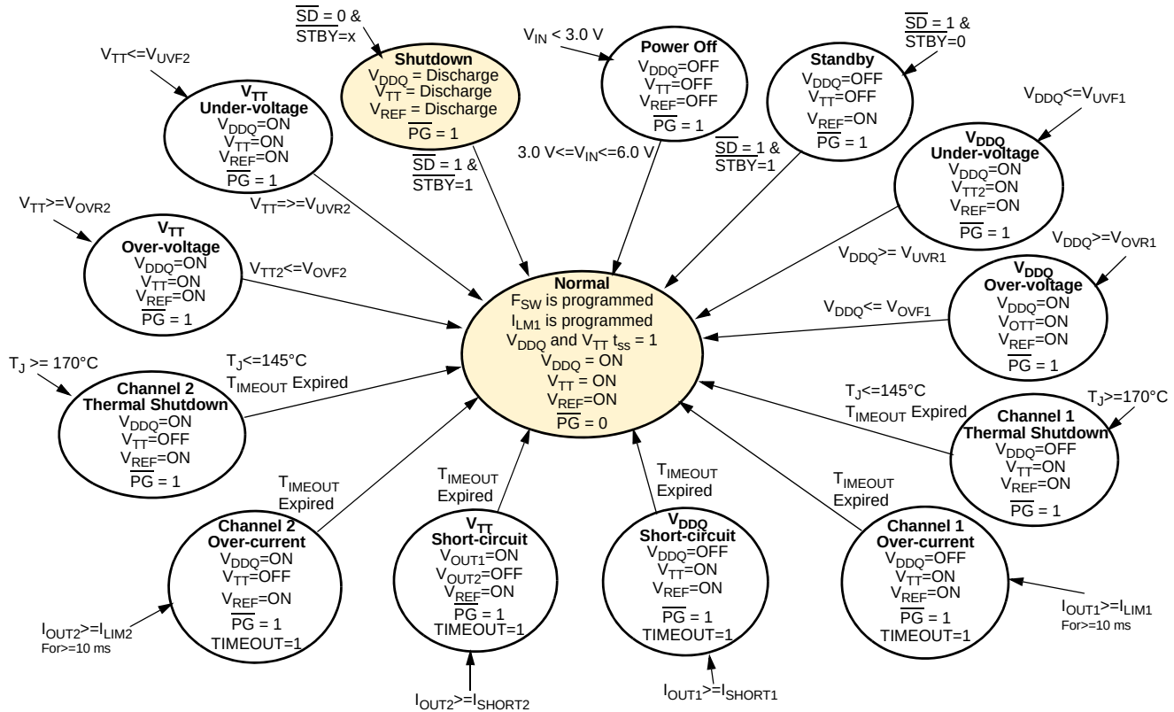
Figure 8. Operation Modes Diagram
