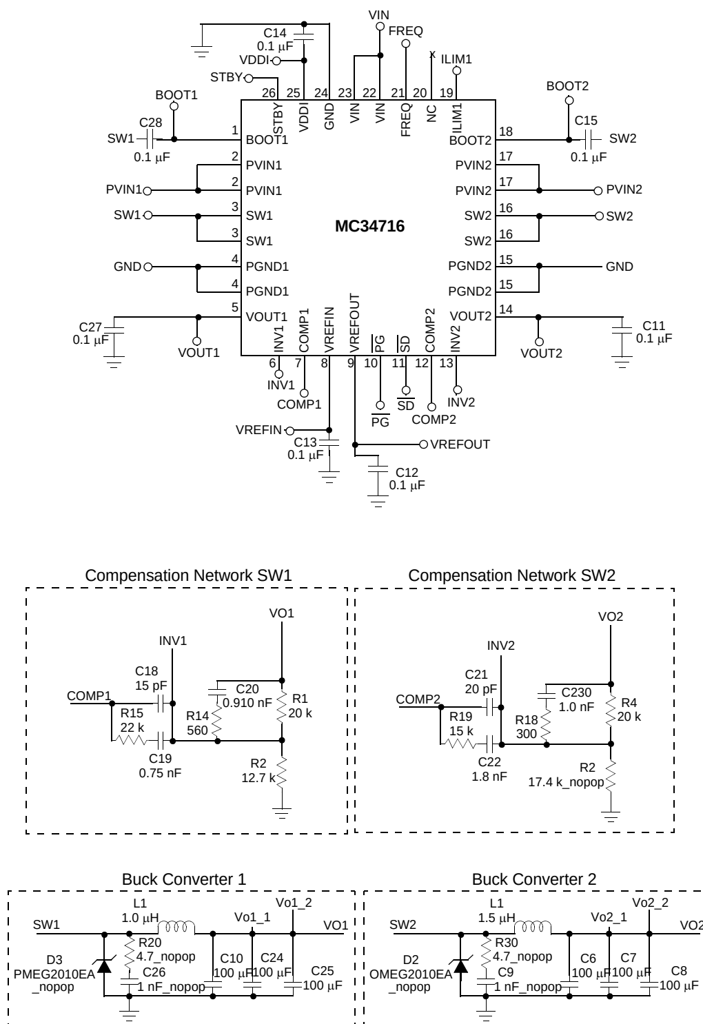
Figure 9. 34716 Typical Application
