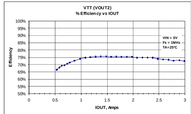
Figure 5. % Efficiency vs. I_{\text{OUT}}
