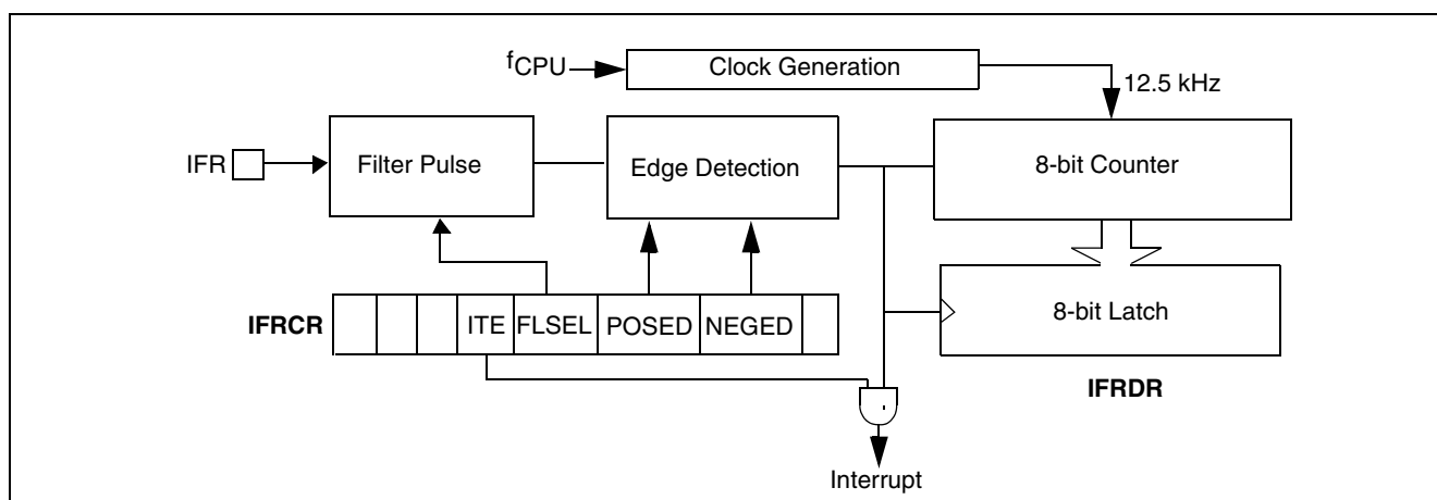
Figure 43: IFR Block Diagram
