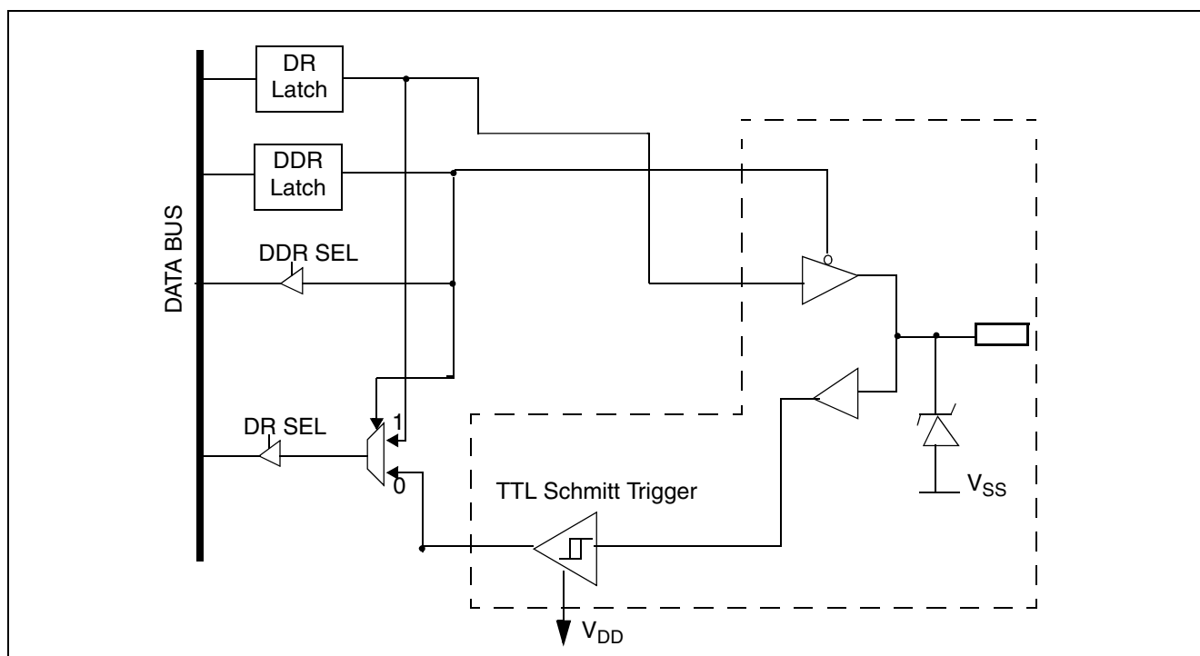
Figure 21: Port C
