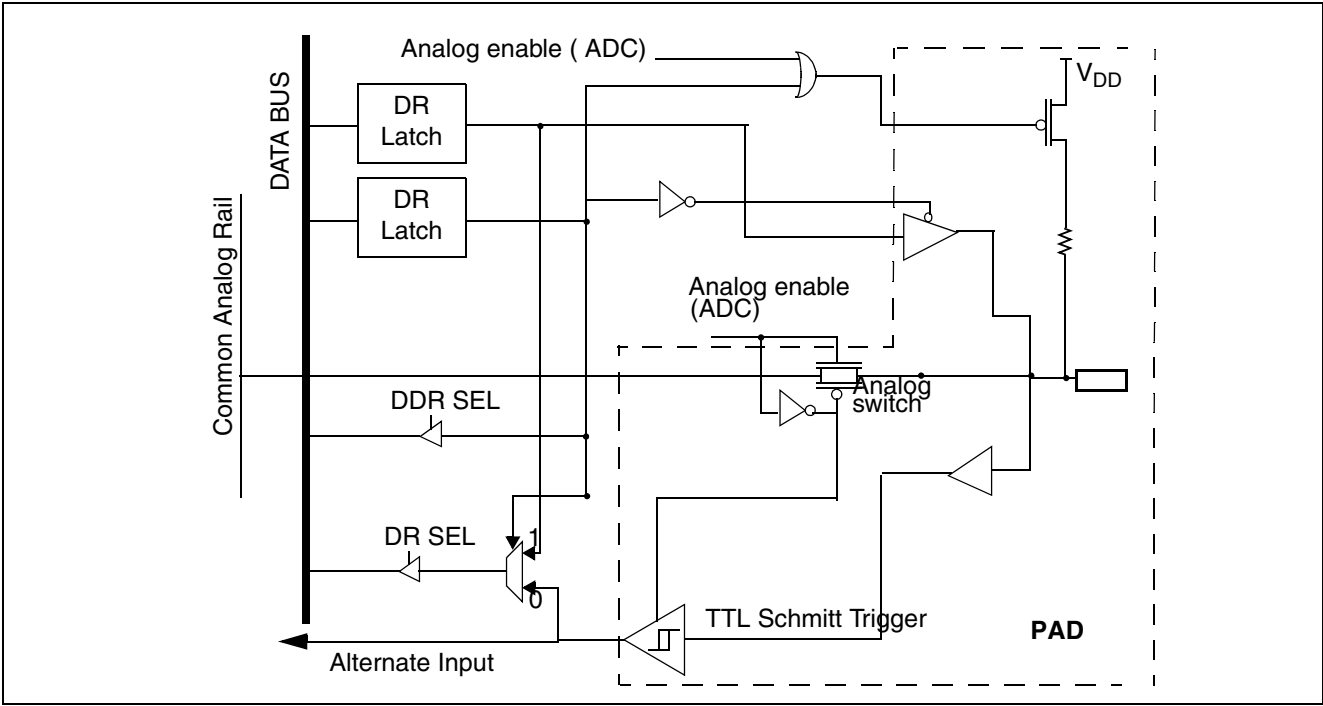
Figure 20: Port B [3]
