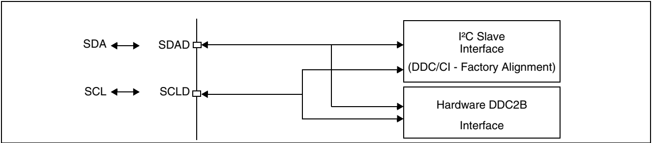
Figure 33: DDC Interface Block Diagram
