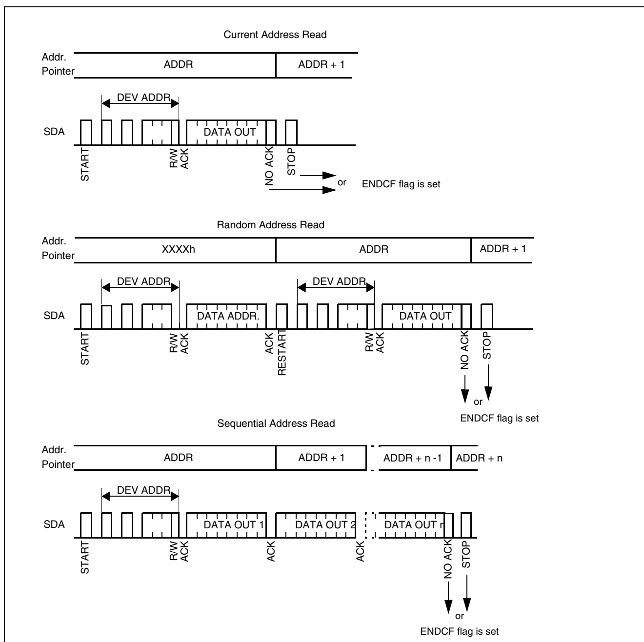
Figure 38: Read Sequences
