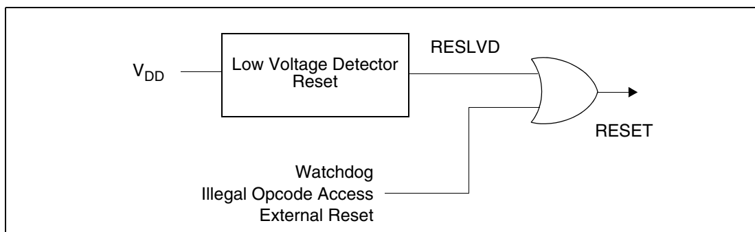
Figure 8: Reset Generation Diagram
