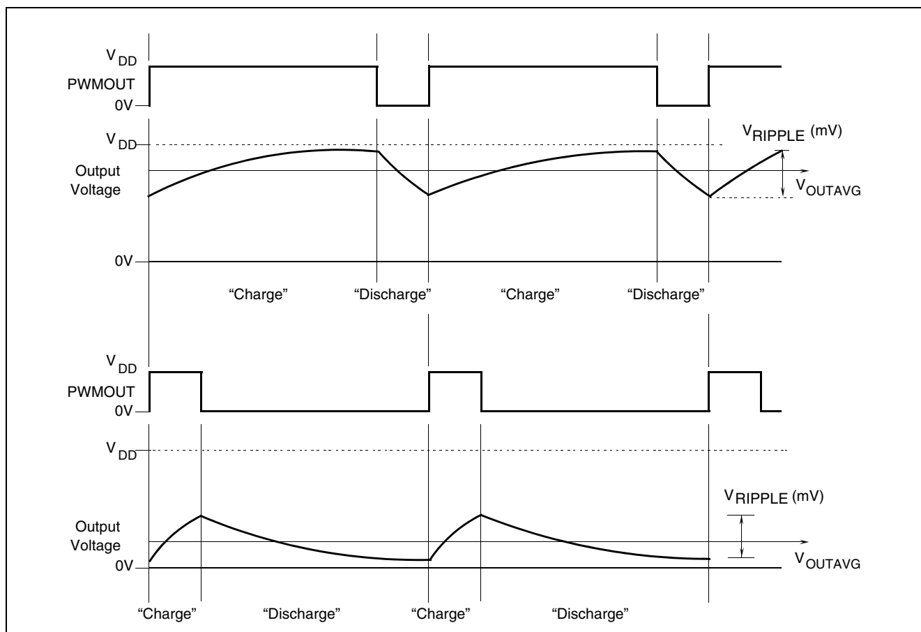
Figure 26: PWM Simplified Voltage Output after Filtering
