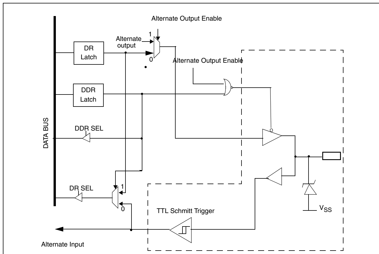
Figure 22: Port D
