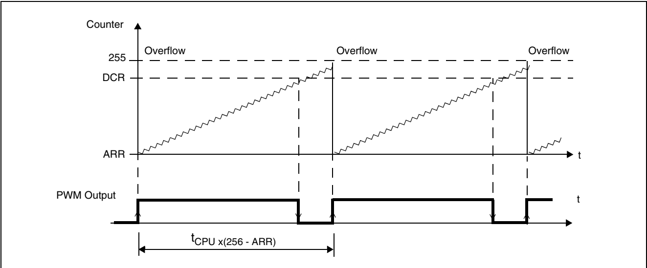
Figure 24: PWM Generation
