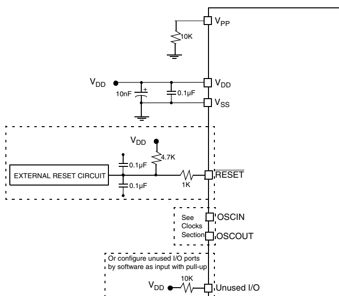
Figure 3: Recommended External Connections
