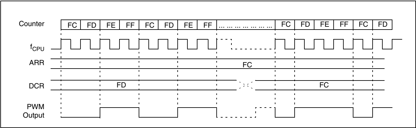
Figure 25: PWM Generation
