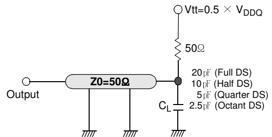
Figure 2. AC Output Load Circuit
