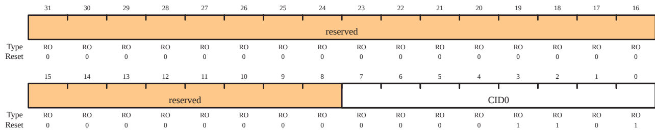
GPIO Primecell Identification 0 (GPIOCellID0) Offset 0xFF0
