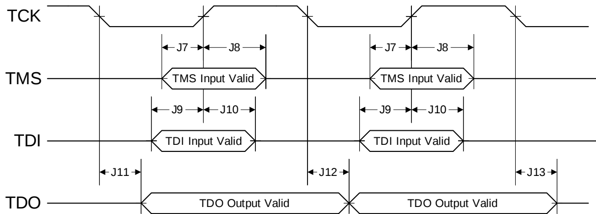
Figure 19-6. JTAG Test Access Port (TAP) Timing
