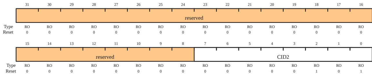
GPIO Primecell Identification 2 (GPIOCellID2)
