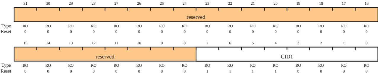
GPIO Primecell Identification 1 (GPIOCellID1) Offset 0xFF4
