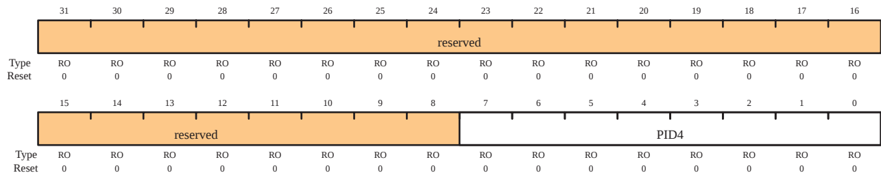
GPIO Peripheral Identification 4 (GPIOPeriphID4) Offset 0xFD0
