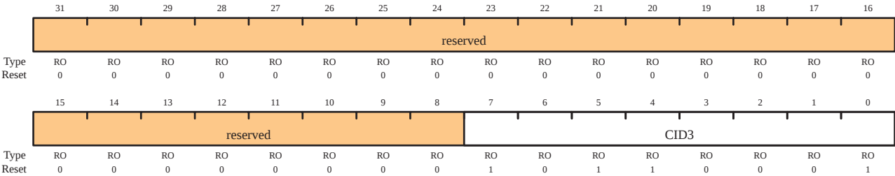
GPIO Primecell Identification 3 (GPIOCellID3)
