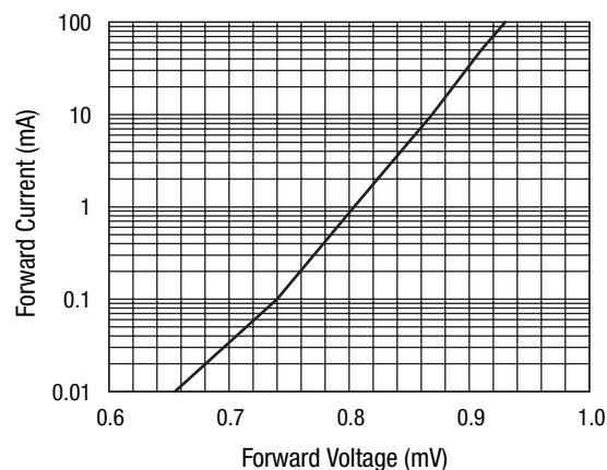
DC Characteristic
