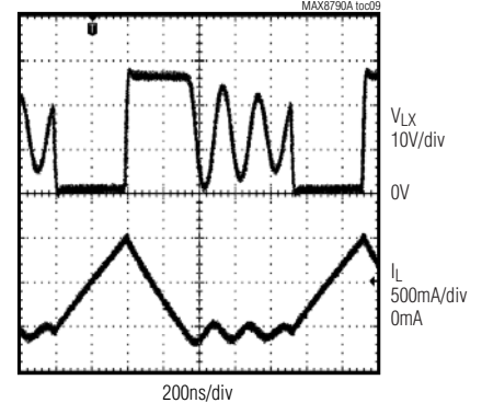
SWITCHING WAVEFORMS (BRT = 100%)
