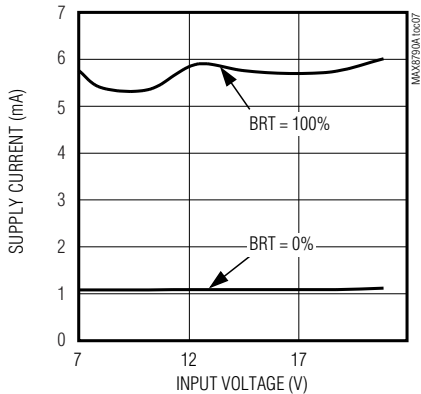
SUPPLY CURRENT vs. INPUT VOLTAGE (DPWM DIMMING)
