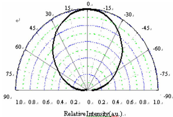
Radiation Characteristics
