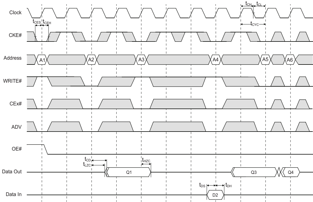
FIG. 5 TIMING WAVEFORM OF CKE# OPERATION
