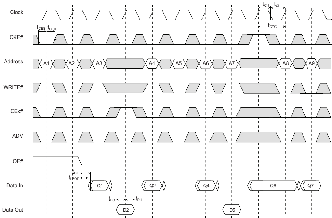
FIG. 4 TIMING WAVEFORM OF SINGLE READ/WRITE
