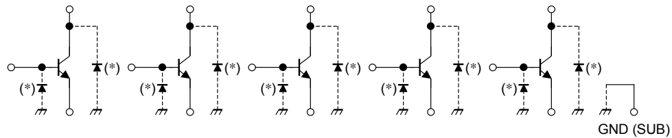
TD62507PG/FG
