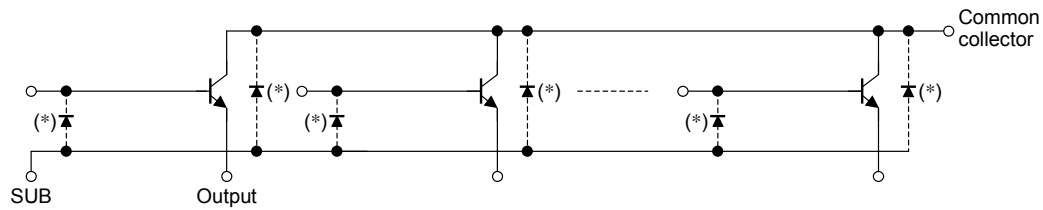
TD62505PG/FG
