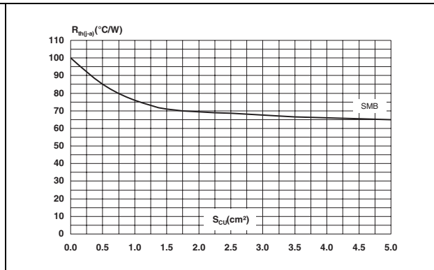
Figure 14. Thermal resistance, junction to ambient, versus copper surface under each lead - SMB (Epoxy FR4, copper thickness = 35 \mu m)
