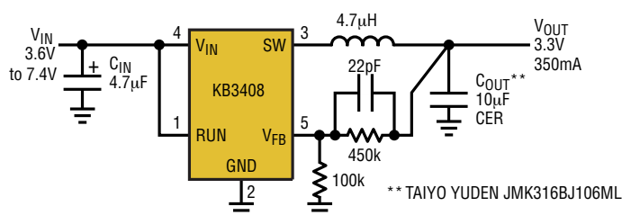
Tiny 3.3V/350mA Buck Regulator
