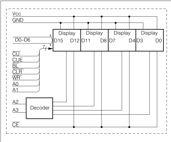
Figure 6. General interface circuit
