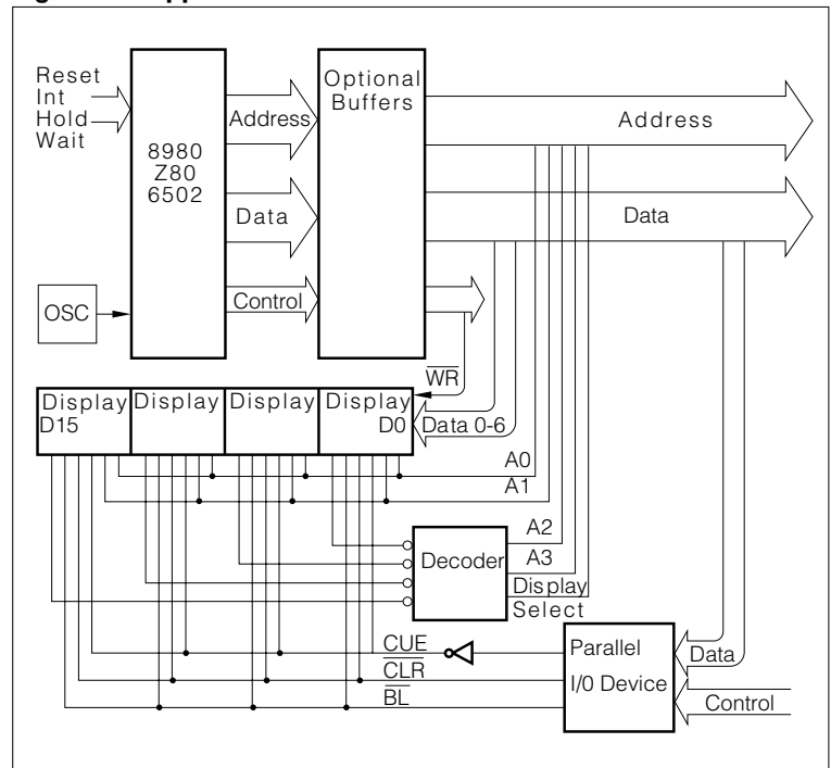
Figure 8. Mapped interface
