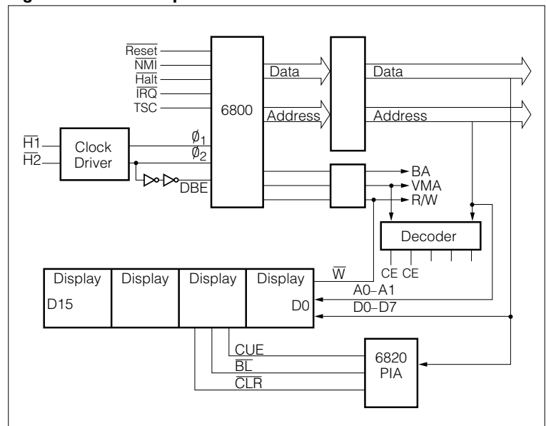
Figure 9. 6800 microprocessor interface
