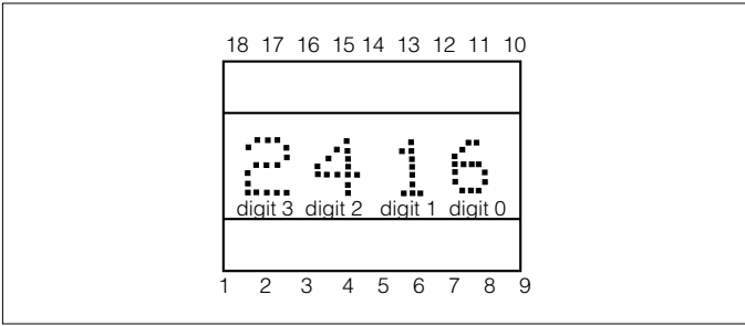
Figure 2. Top view and pin outs
