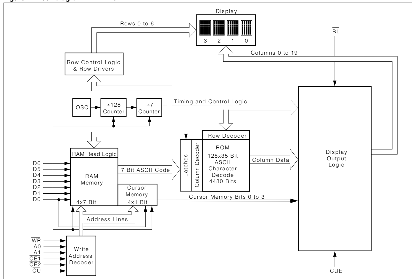
Figure 1. Block diagram–DLX2416
