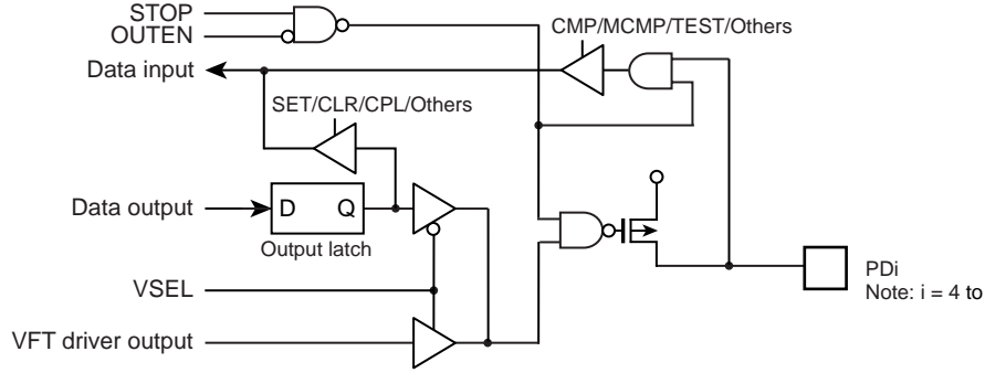
Figure 5-9 Port PD
