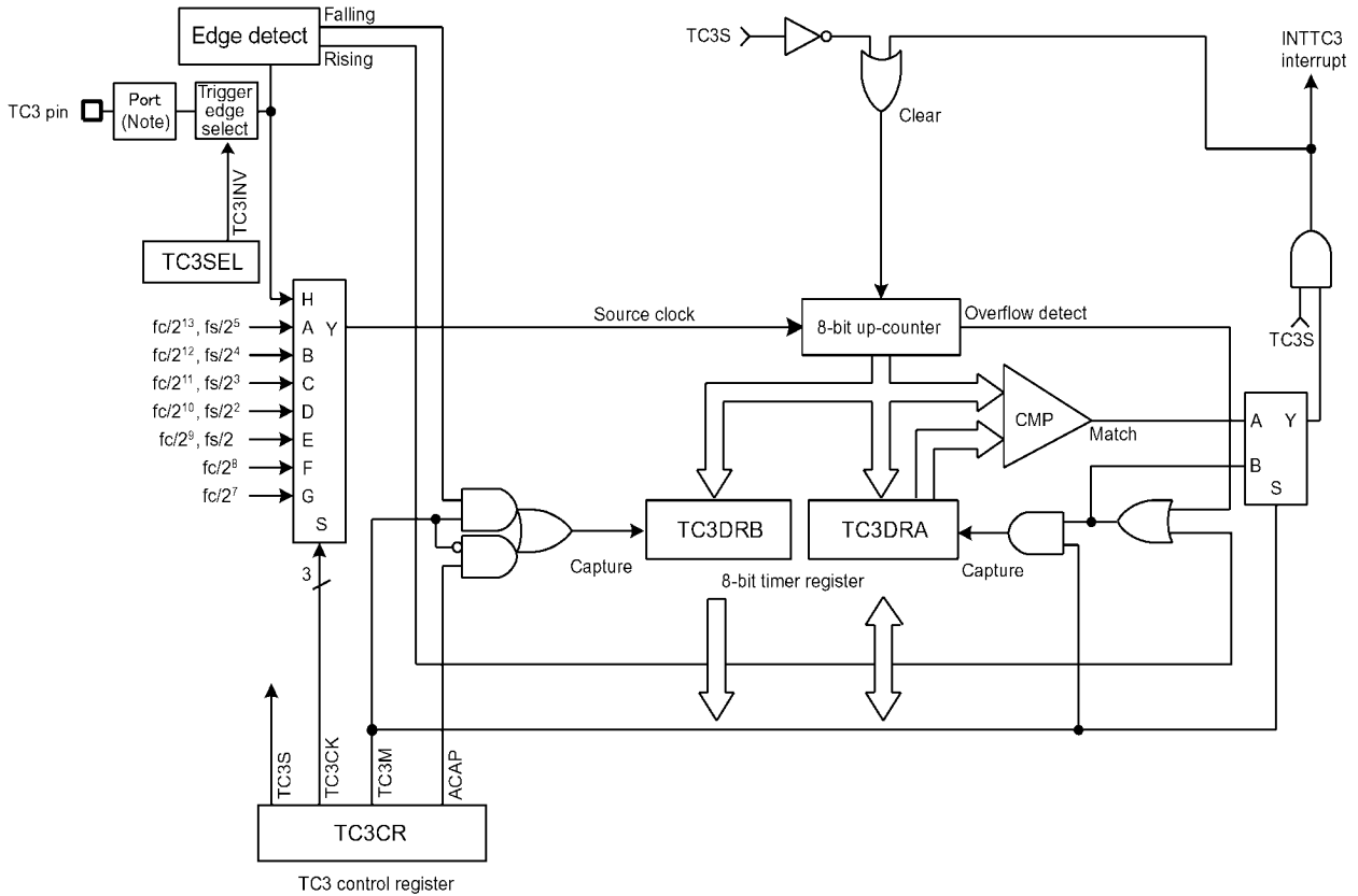
Figure 10-1 TimerCounter 3 (TC3)
