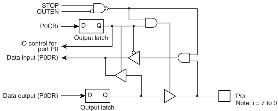
Figure 5-2 Port P0
