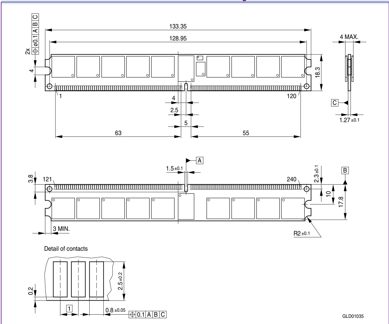
Package Outline Raw Card XX - L-DIM-240-54
