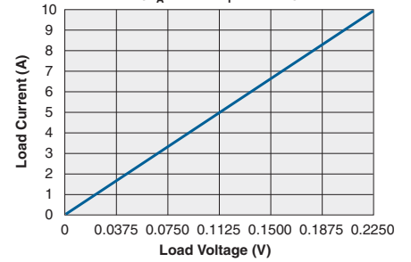
CPC1709 Typical Load Current vs. Load Voltage ( T_A = 25°C, I_F = 10mA )
