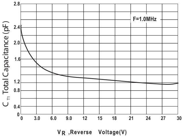
Figure 1 .Total Capacitance
