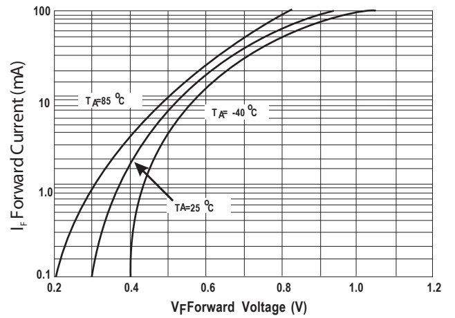
Figure 4 .Forward Voltage
