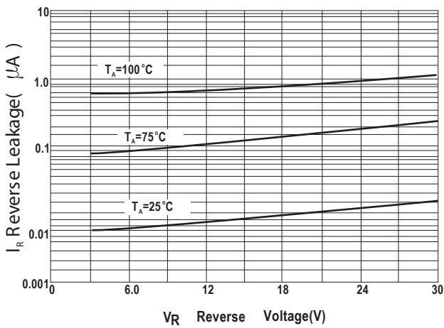
Figure 3 .Reverse Leakage
