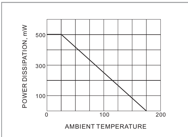
Fig.4 DERATING CURVE
