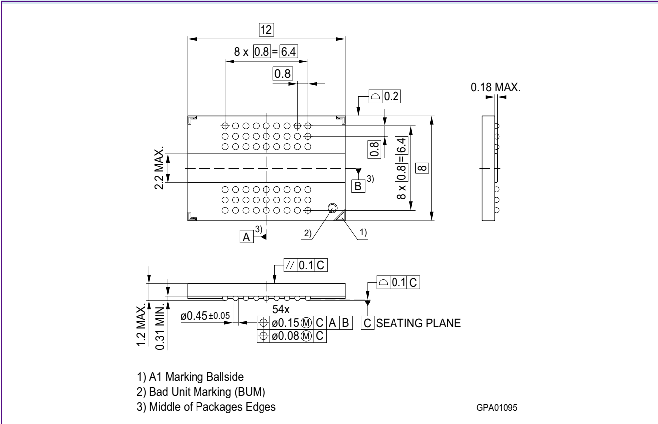
FIGURE 6 Package Outline PG-TFBGA-54-15
