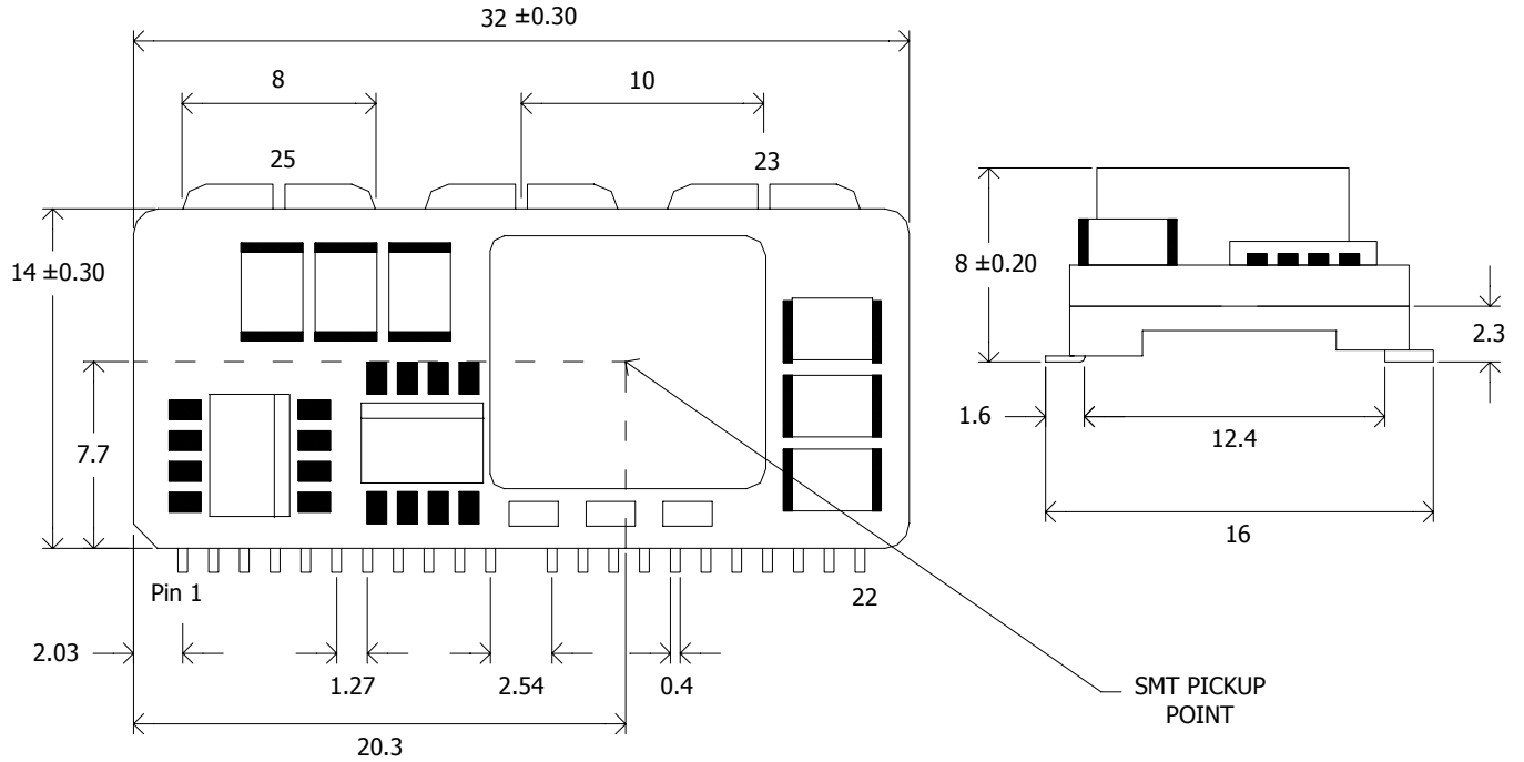
Figure 58. Mechanical Drawing
