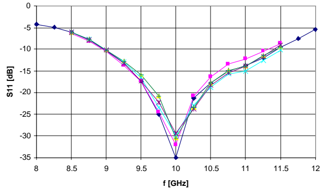
Input return loss ( V_d=8V , V_{gg}=-5V , P_s=17dBm )
