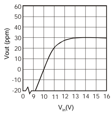
CHANGE IN OUTPUT VOLTAGE VS. INPUT VOLTAGE
