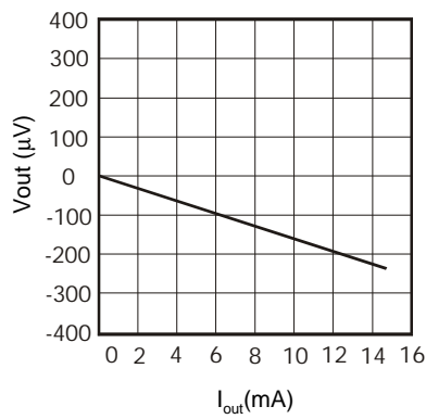
CHANGE IN OUTPUT VOLTAGE VS. OUTPUT CURRENT
