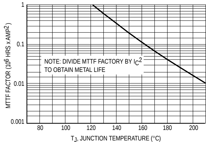
Figure 4. MTTF Factor versus Junction Temperature
