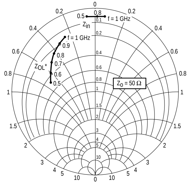
Figure 2. Large Signal Impedances V CE = 20 V — I C = 440 mA
