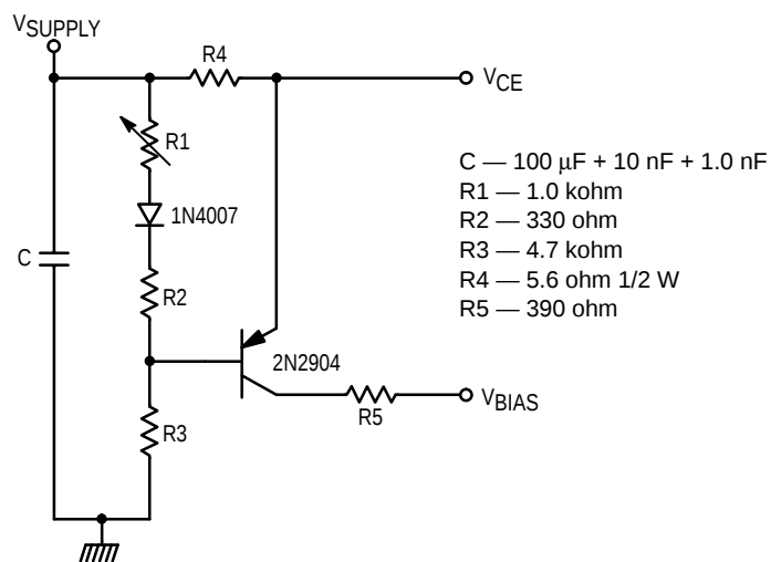
Figure 6. Class A Bias Circuit
