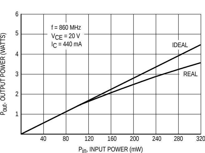
Figure 1. Power Output versus Power Input
