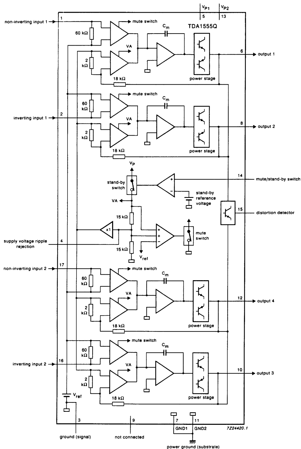
Fig.1 Block diagram.
