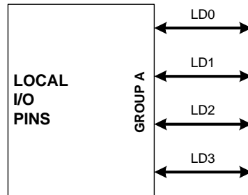
GROUP A CONFIGURATION AT 2.048, 4.096, OR 8.192 Mb/s
