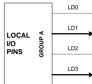
GROUP A CONFIGURATION 4 AT 16.384 Mb/s SUPERRATE
