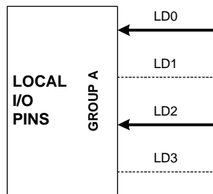
GROUP A CONFIGURATION 1 AT 16.384 Mb/s SUPERRATE
