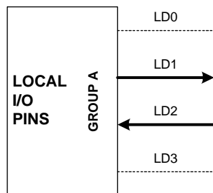
GROUP A CONFIGURATION 3 AT 16.384 Mb/s SUPERRATE
