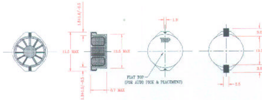
PCB PATTERN
