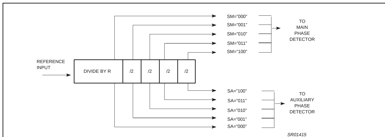
Figure 5. Reference Divider
