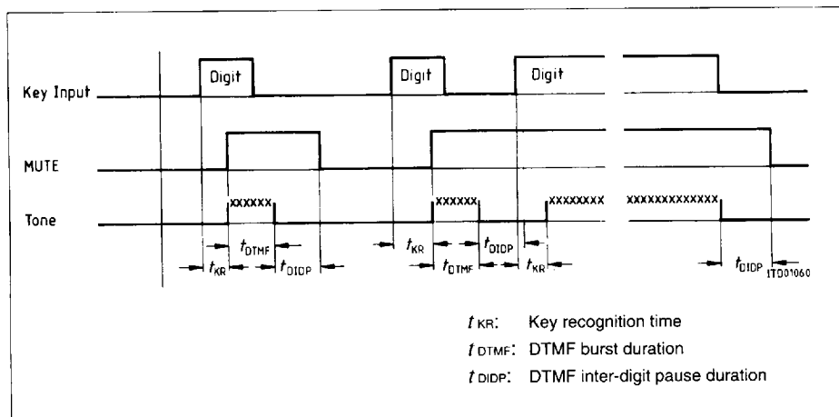
Figure 2 DTMF-Dialing
