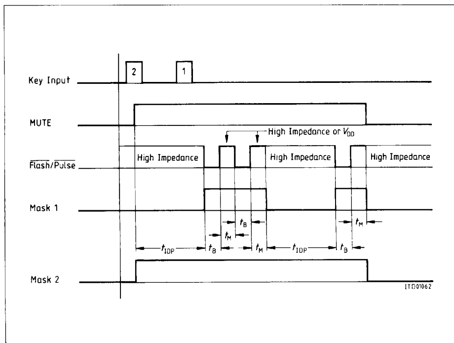
Figure 4 Pulse Dialing
