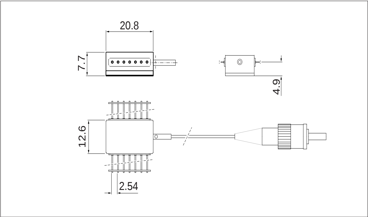
Figure 1. Mechanical outline
