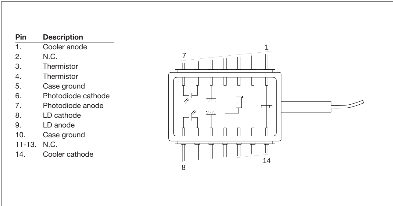
Figure 2. Pin description
