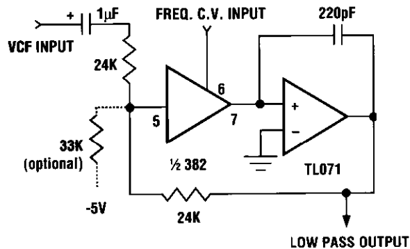
Fig. 2a: 382 in first order low pass
