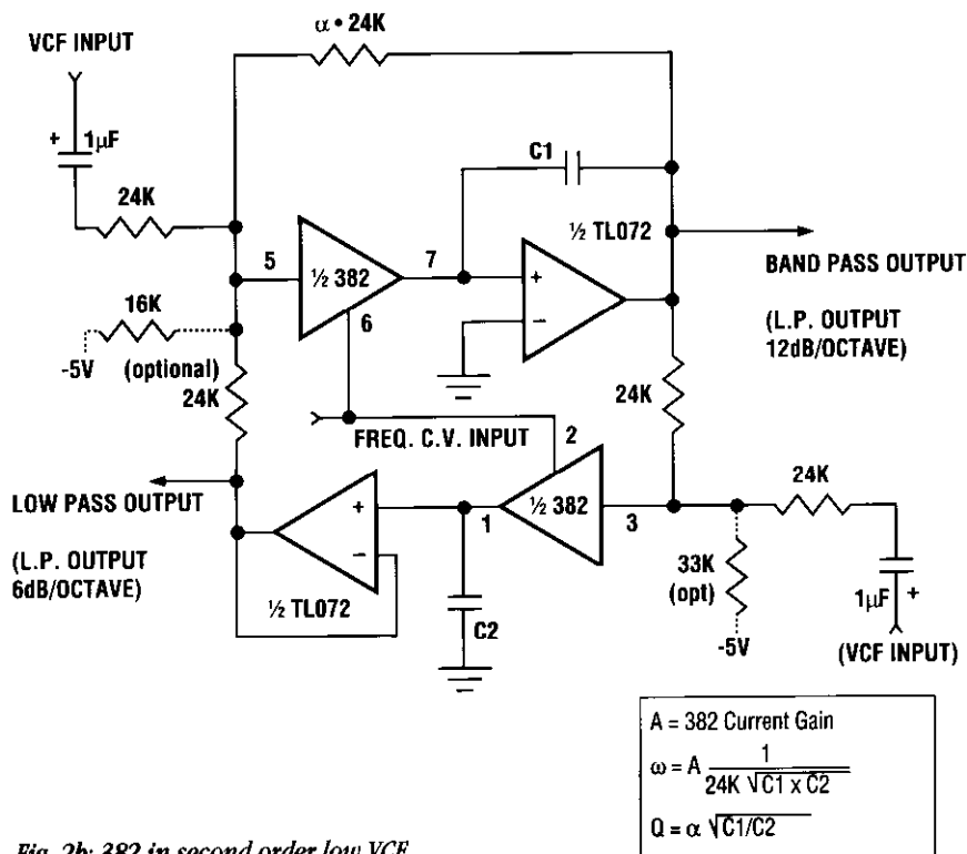
Fig. 2b: 382 in second order low VCF
