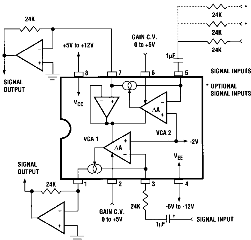
PA 381/382 Block Diagram and Typical Connection
