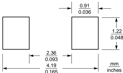
SOD-123
