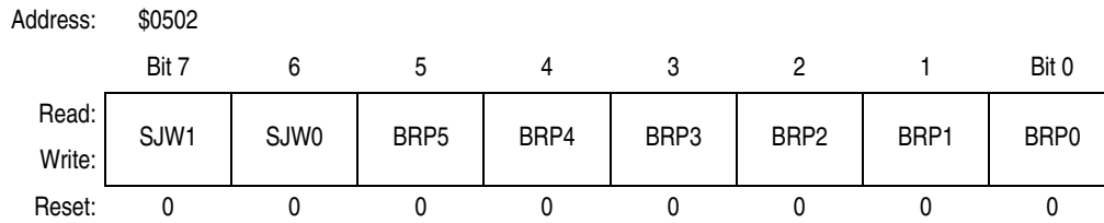
Figure 24-17. Bus Timing Register 0 (CBTR0)
