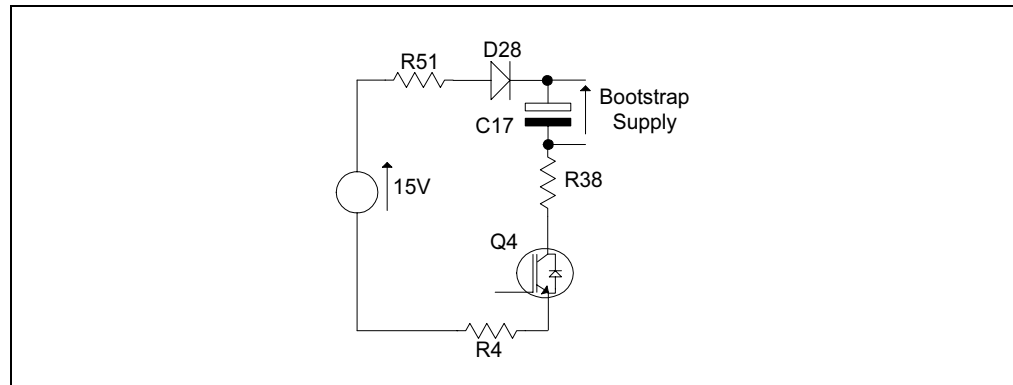
FIGURE 1-7: BOOTSTRAP SUPPLY
