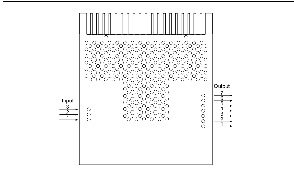
FIGURE 1-3: POWER CONNECTIONS
